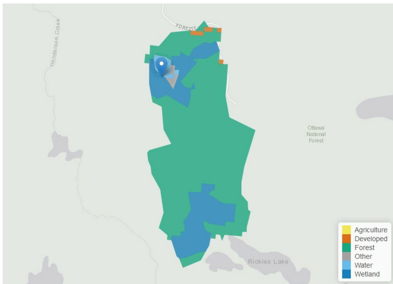
Figure 1. Land use map of Raven Lake.
