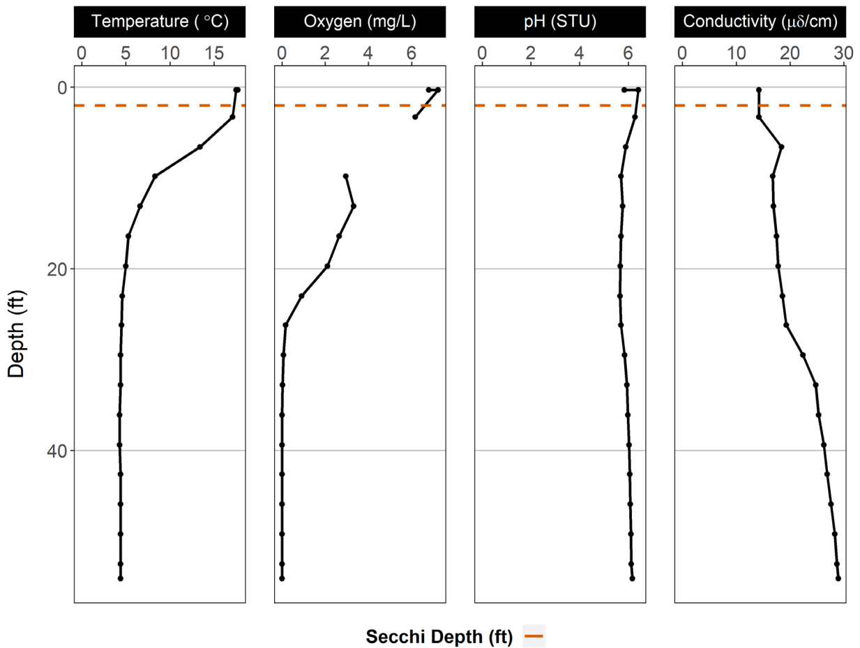
Figure 2. Vertical profile of temperature, dissolved oxygen, pH, and conductivity collected during the 2017 National Lakes Assessment of Raven Lake.
