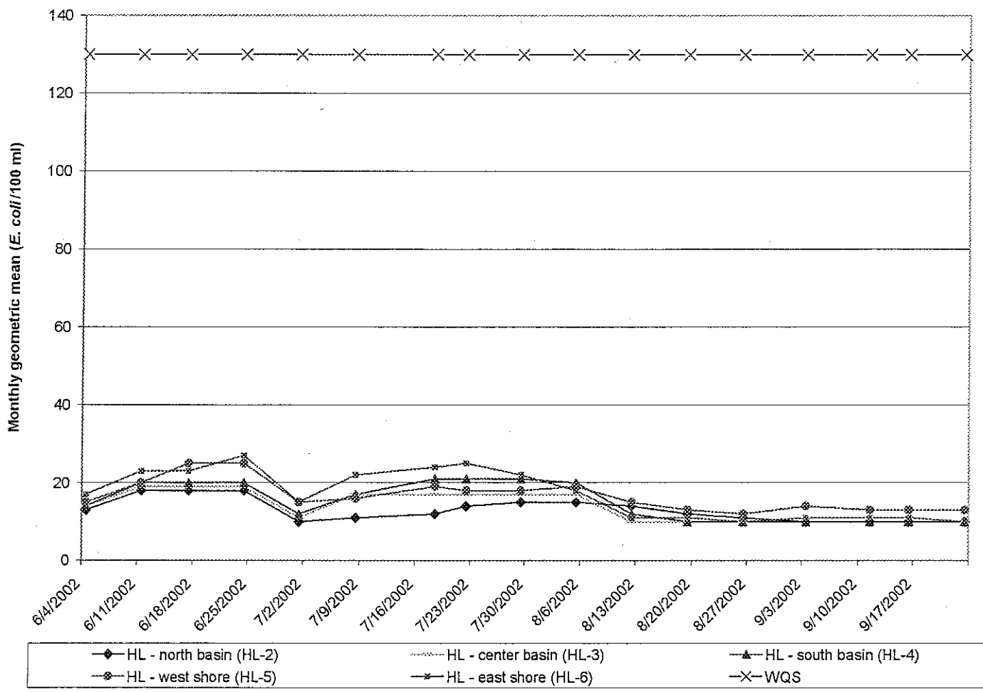
Figure 3. Thirty-day geometric mean for E. coli in Hunter's Lake, vicinity of Glennie, Alcona County, Michigan 2002.
