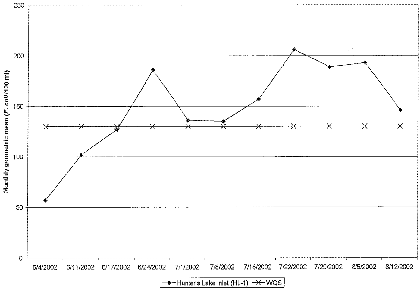
Figure 2. Hunter's Lake inlet E. coli monitoring, vicinity of Glennie, Alcona County, Michigan 2002.
