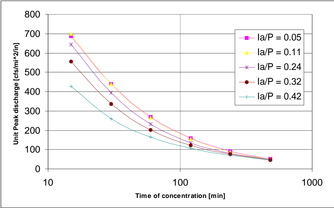
Figure 1 - Unit Peak Discharge Related to Ia/P and Time of Concentration
