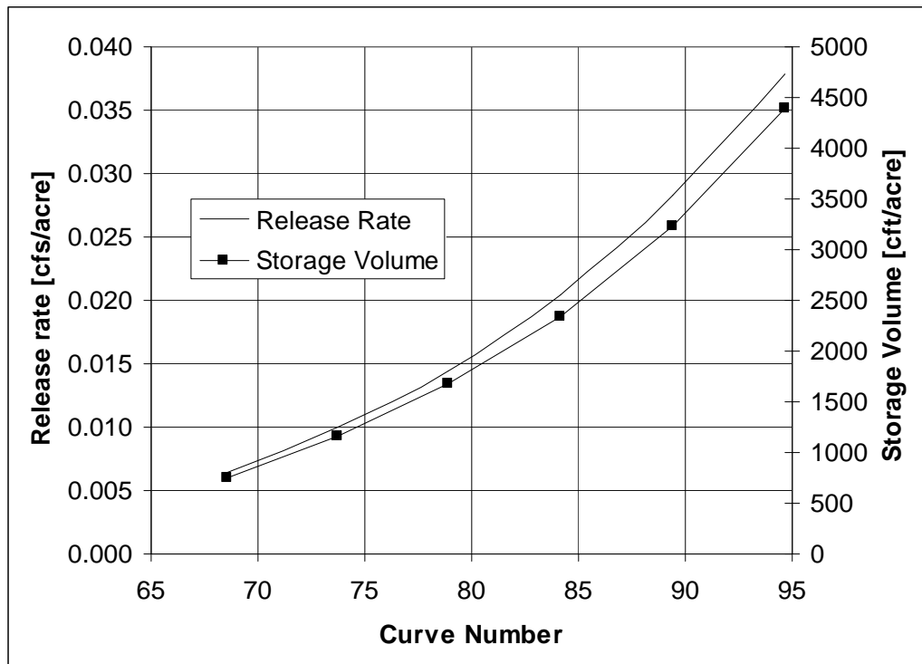
Figure 4 - Release Rate as a Function of Curve Number
