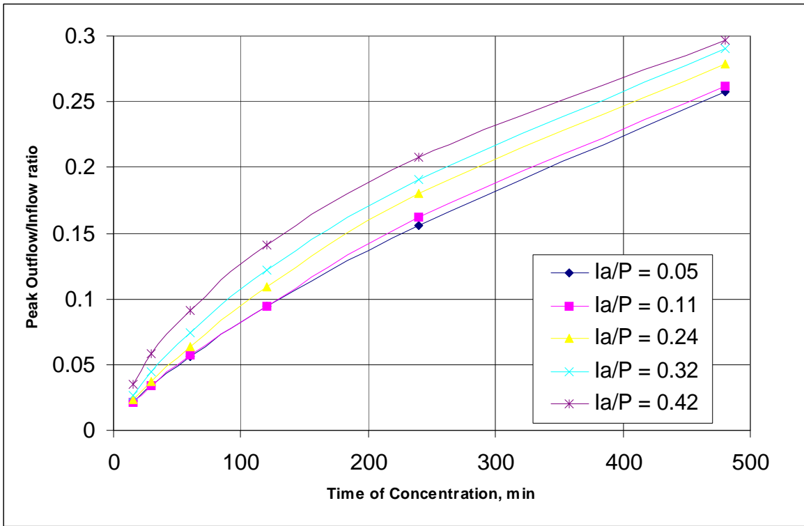
Figure 3 - Peak Inflow/Outflow as a Function of I_a/P and Time of Concentration
