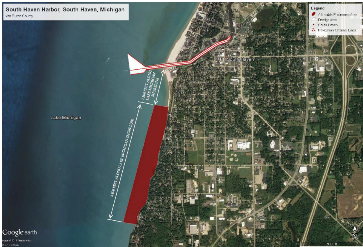
Figure 1. Proposed dredge area within the South Haven Harbor federal navigational channel and beach nourishment placement location along the Lake Michigan shoreline.
