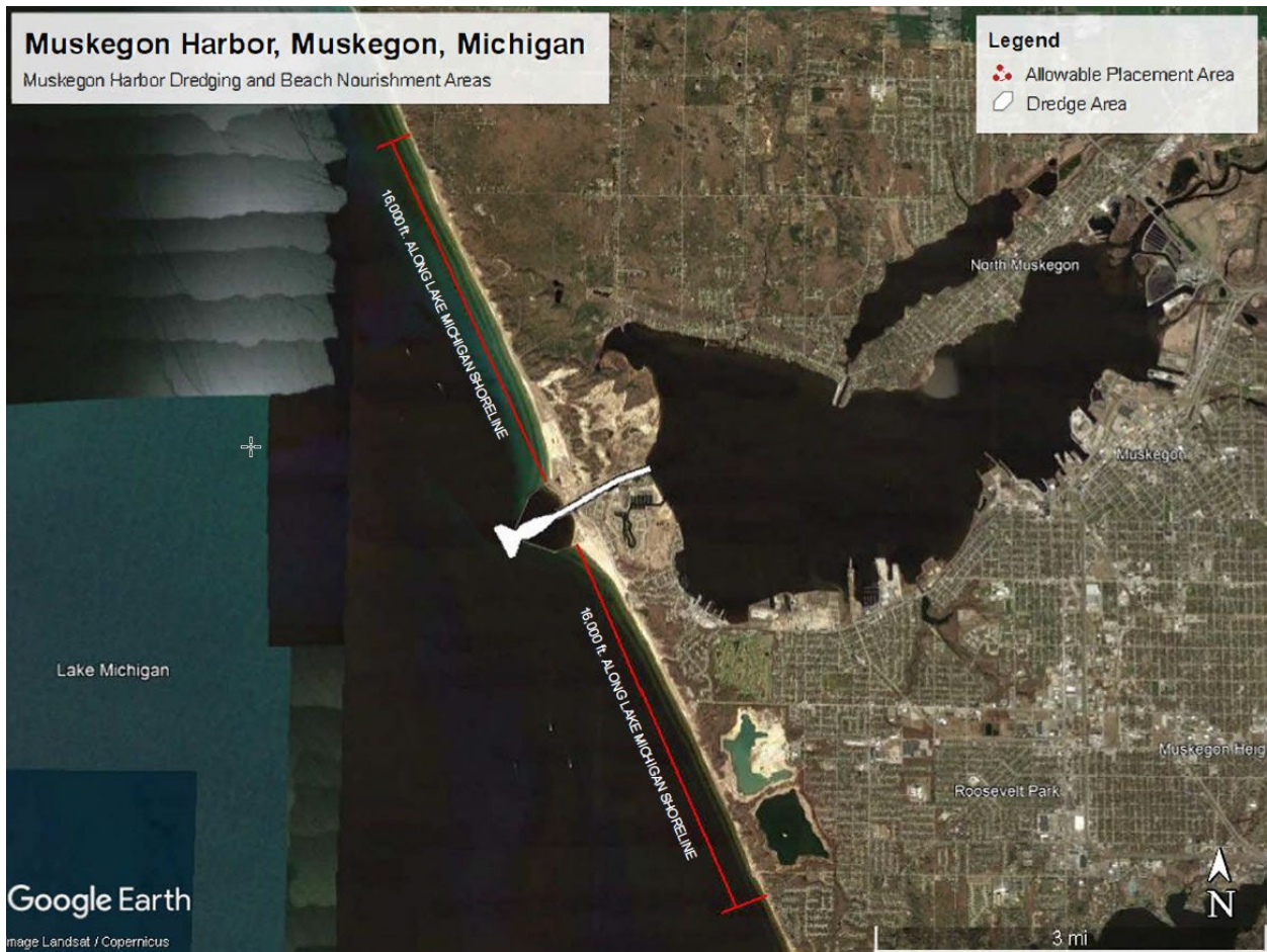
Figure 1. Muskegon Harbor dredging and beach nourishment areas.
