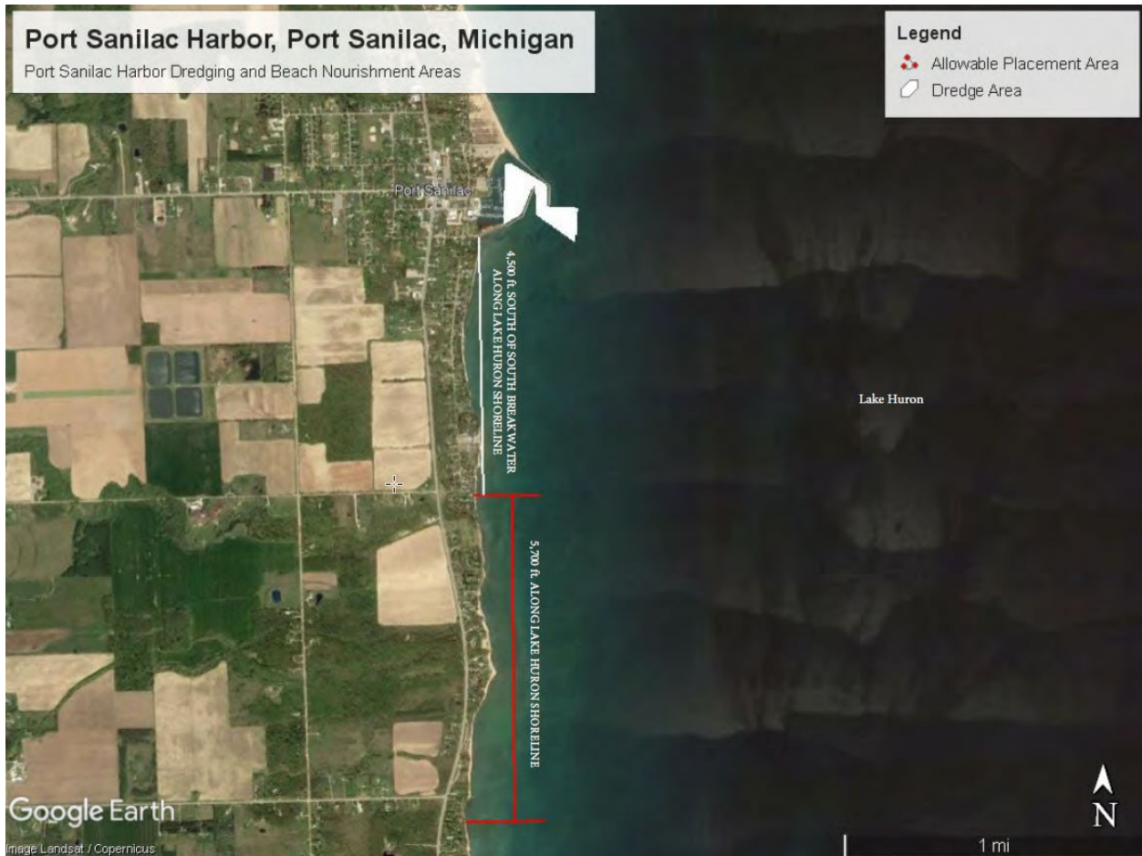
Figure 1. Port Sanilac Harbor dredging and beach nourishment areas.
