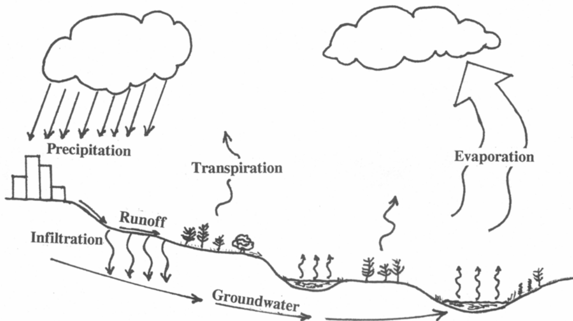
Figure 1.1 Hydrologic Cycle
