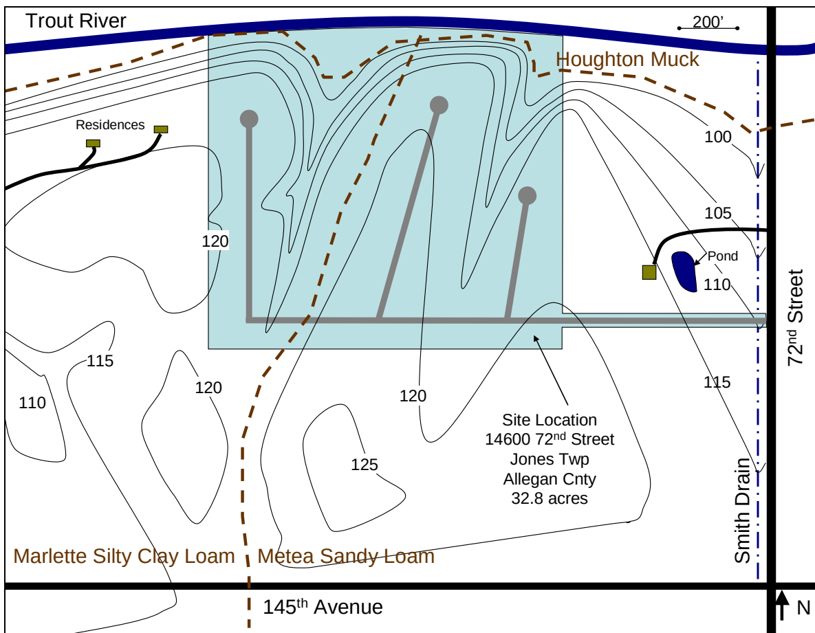
Figure 10-9: Site Location Sketch and Soils Information
