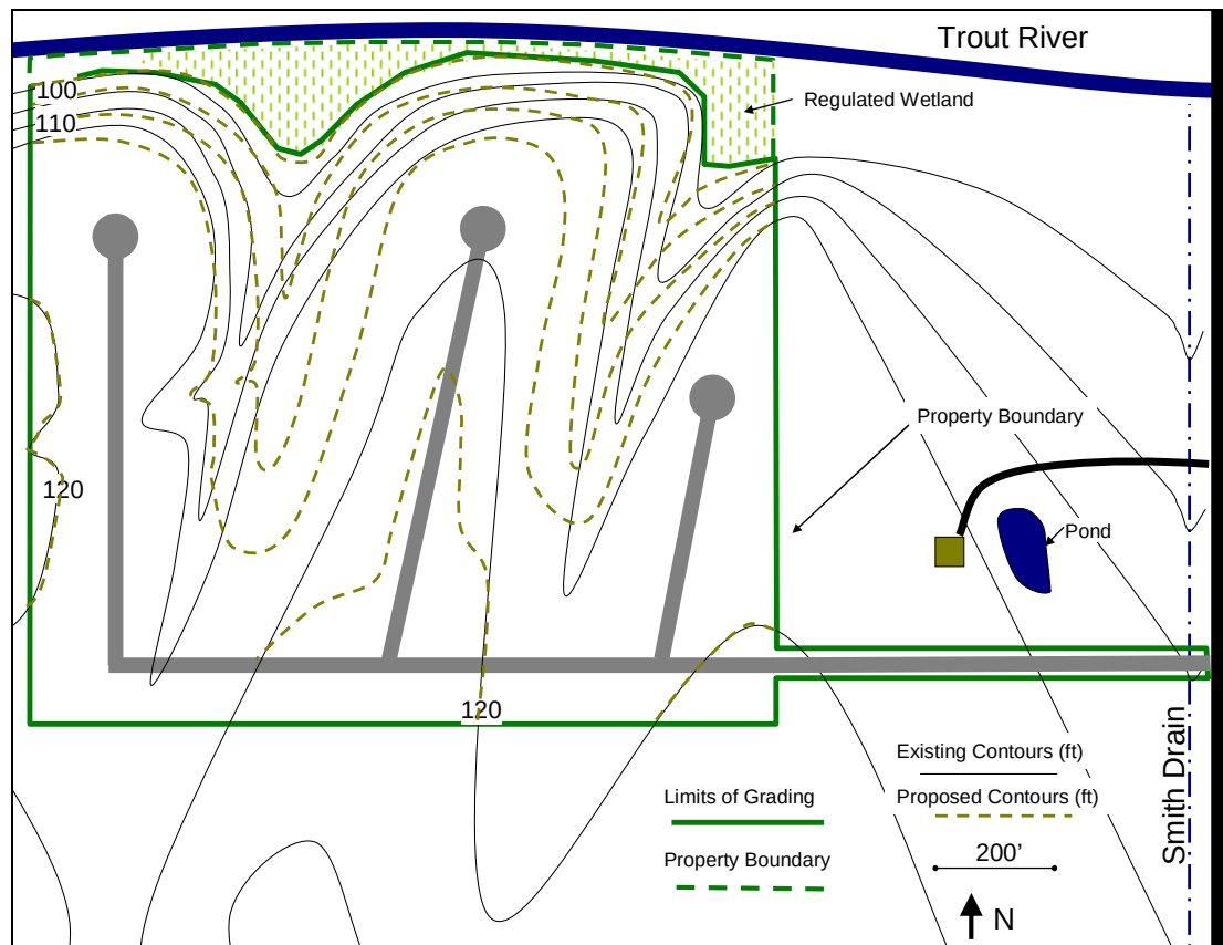
Figure 10-3: Rough grading map for proposed development
