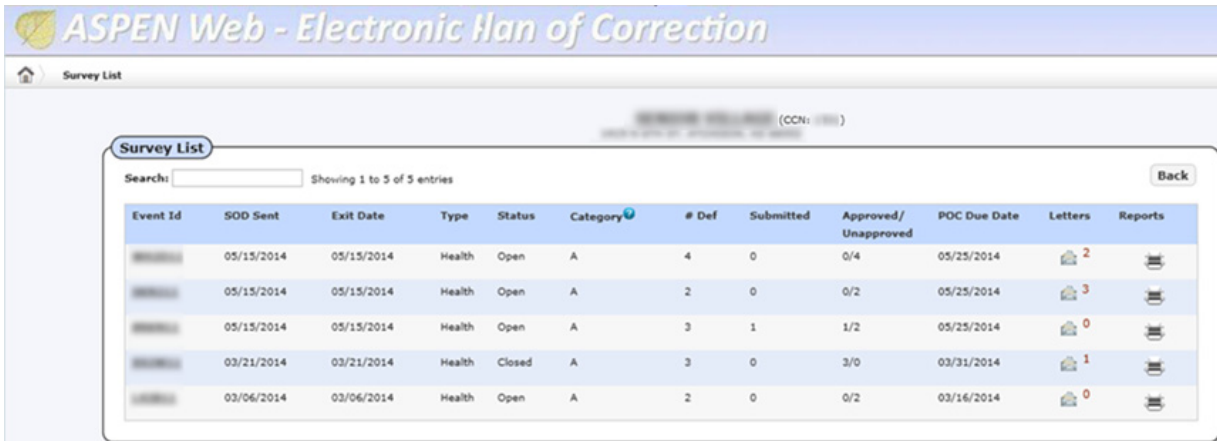
Figure 17: Survey List
