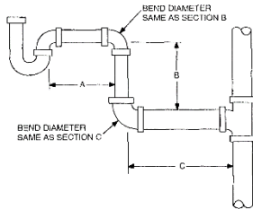
FIGURE P3105.4 VERTICAL LEG FIXTURE DRAIN SCHEMATIC
