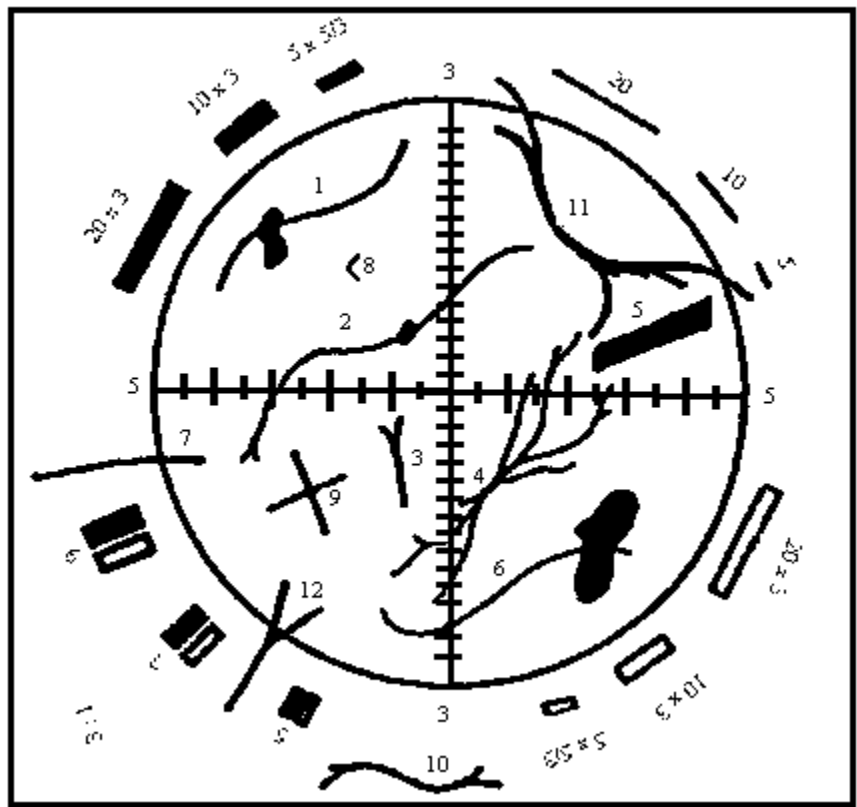
Figure 1: Walton-Beckett Graticule with some explanatory fibers.
