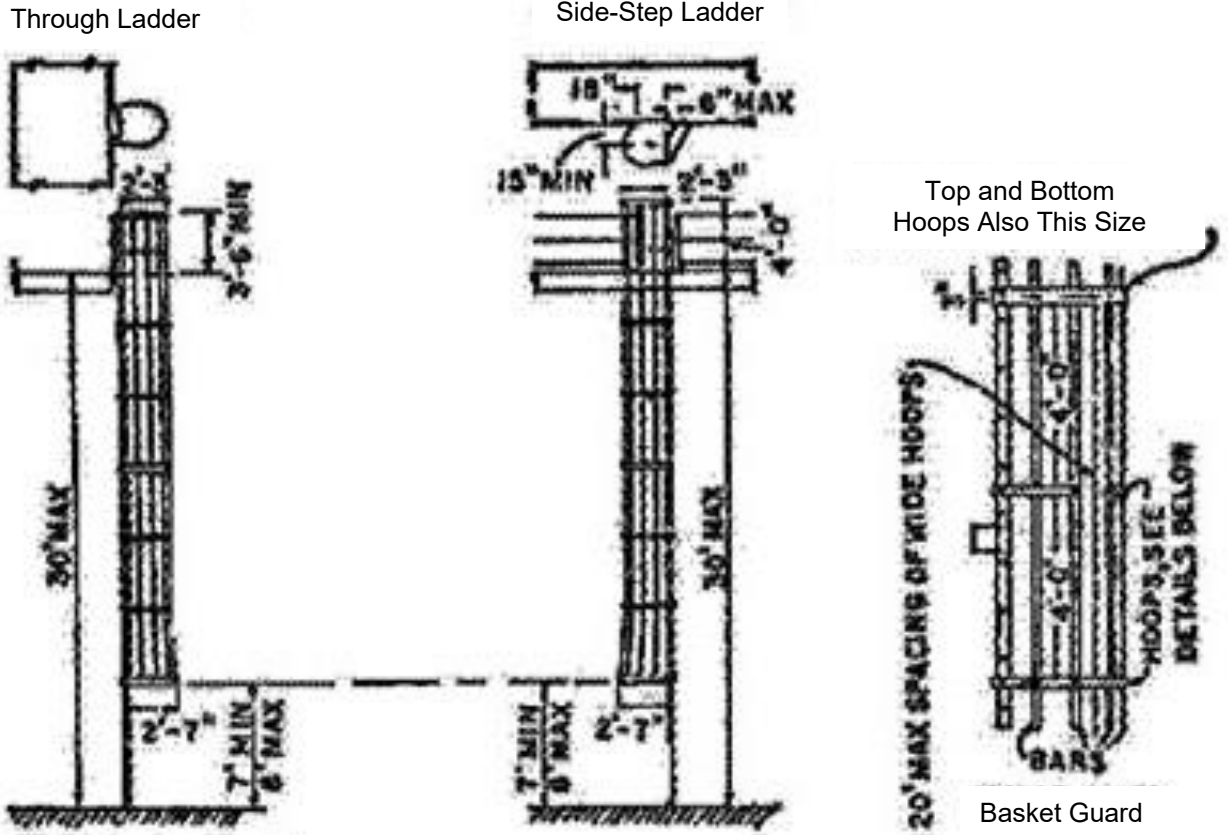
Access Lateral From Ladder
