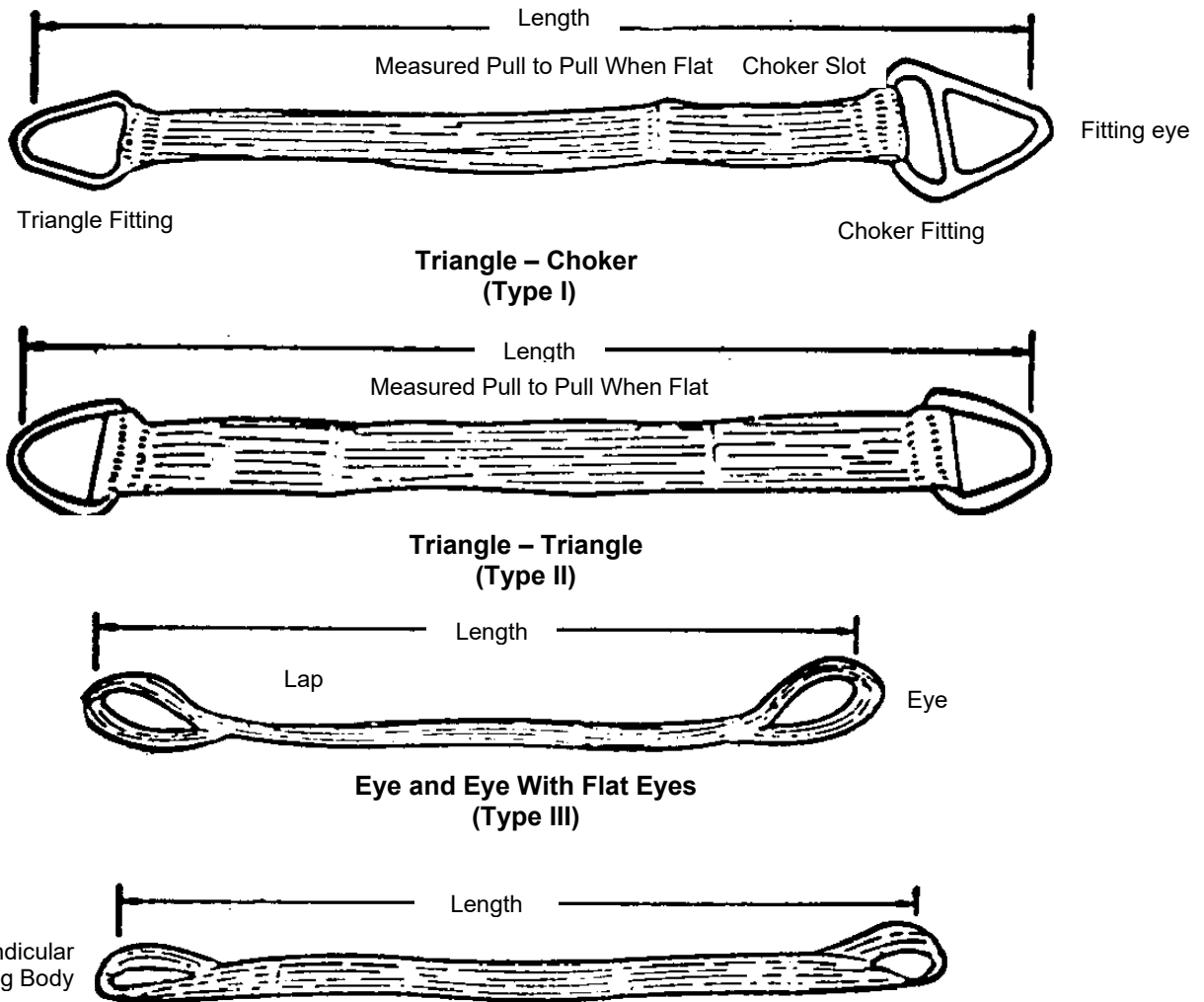
FIGURE 6 BASIC SYNTHETIC WEB SLING CONSTRUCTIONS
