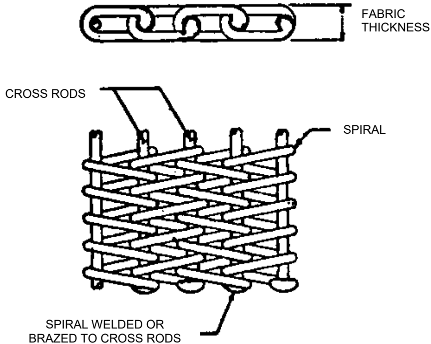
FIGURE 2 METAL MESH CONSTRUCTION
