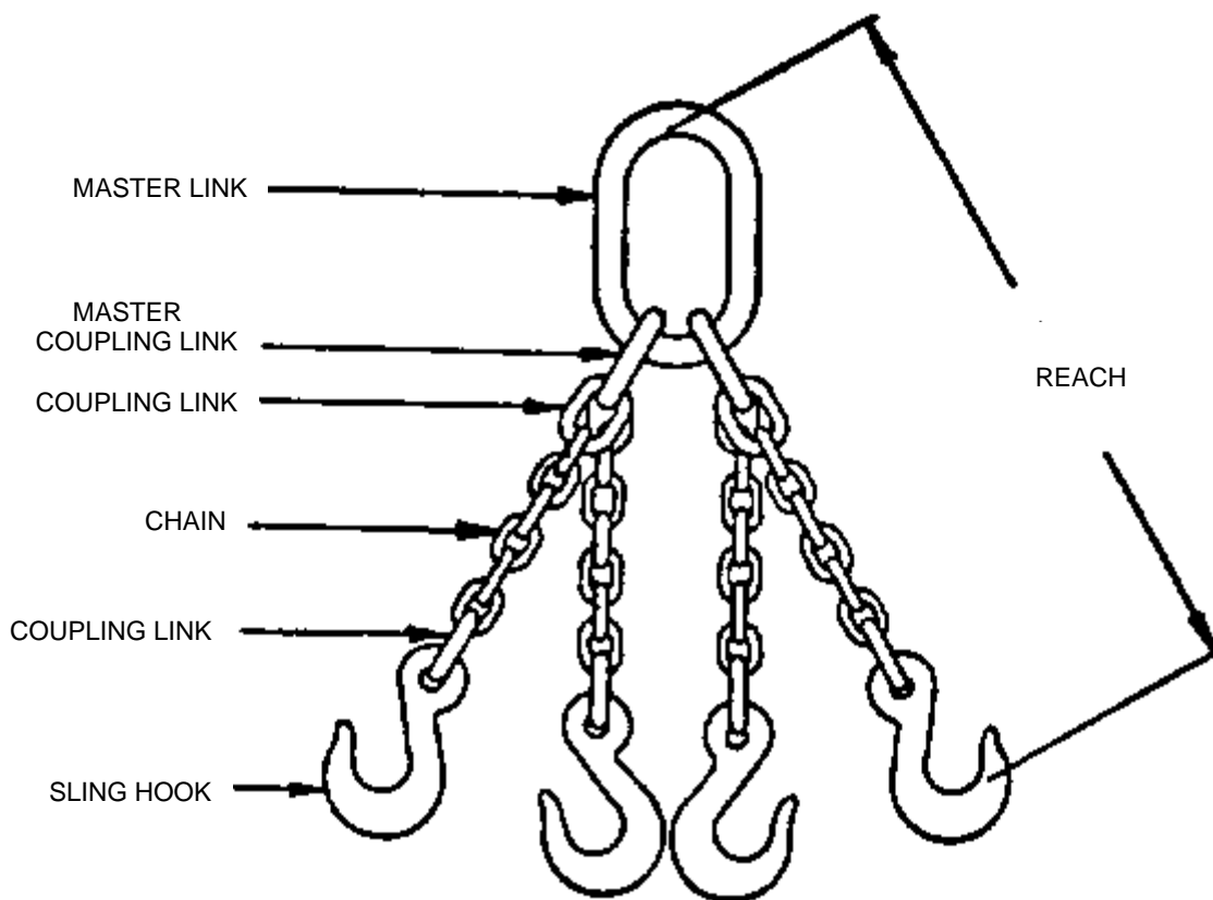
FIGURE 3 MAJOR COMPONENTS OF A GUADRUPLE SLING
