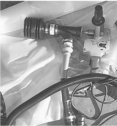
Drill shroud connected to HEPA vacuum: Collect dust where you're generating it.
