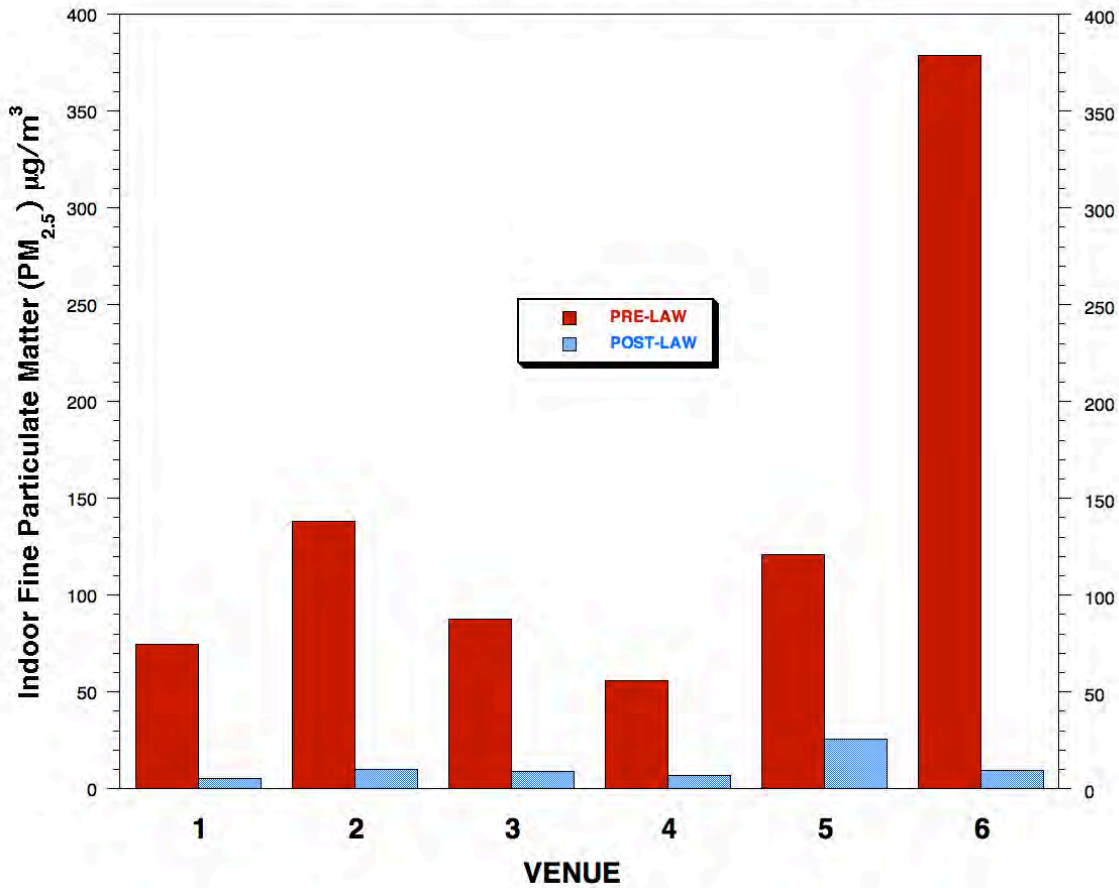
Figure 2. Mean air pollution levels in 6 restaurants, pre-and-post Smoke-free Air Law.
