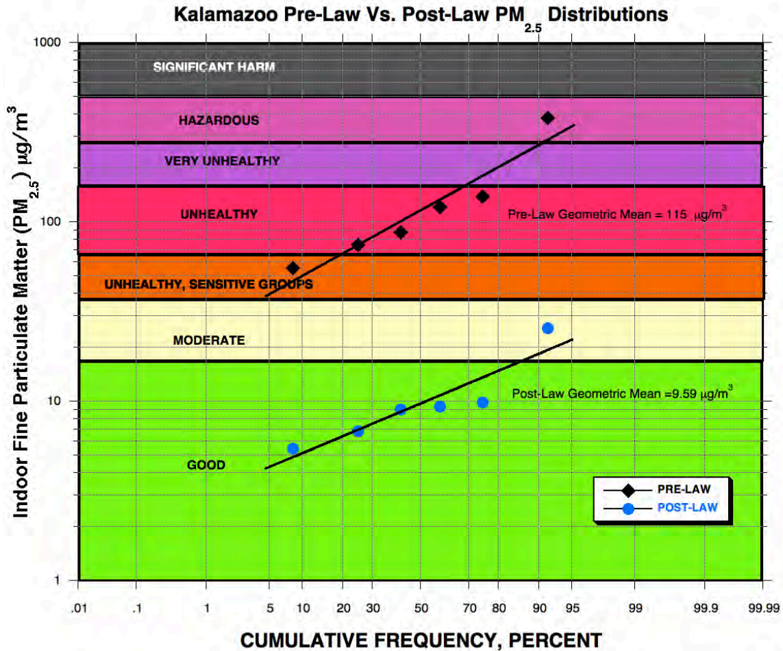
Figure 4. PM 2.5 frequency distributions for 6 Kalamazoo restaurants vs. the Michigan AQI. Pre-law, all 6 venues have very poor air quality. Post-law, all 6 venues have very good air quality.
