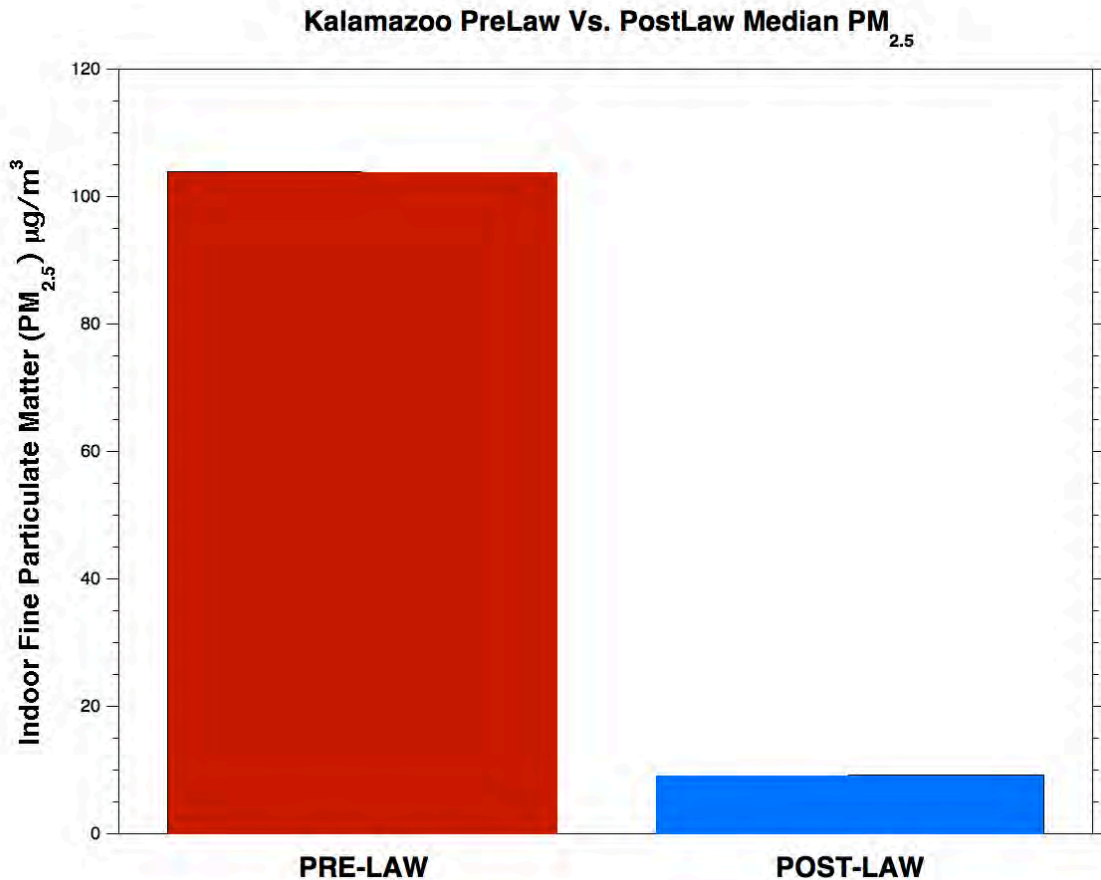
Figure 3. Combined median PM 2.5 level for 6 Kalamazoo restaurants drops an average of 91% due to Michigan’s Dr. Ron Davis Indoor Air Law.
