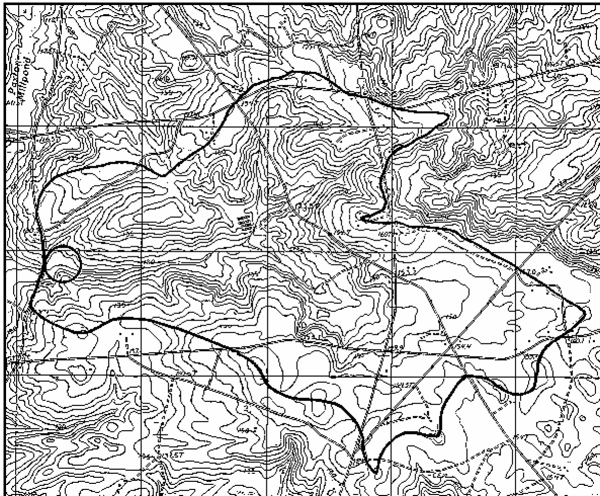
Figure 3.C.1. Topographic Map of Watershed for Example Problem (Dark Line Indicates Drainage Area Boundary)
