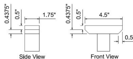
Support Detail
