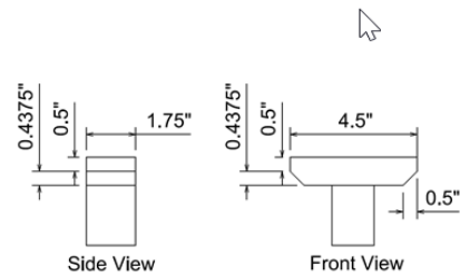
Support Detail
