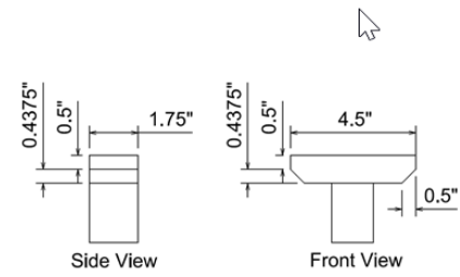
Support Detail
