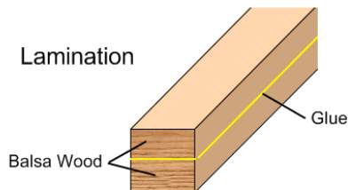
Image 1 Lamination
