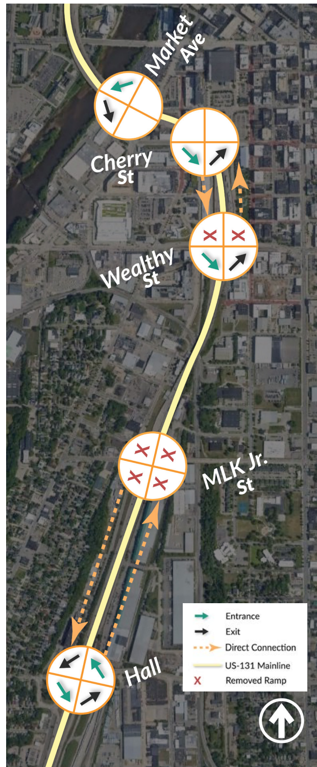
FIGURE 5-5. Cherry Street-to-Hall Street Interchange Option D
