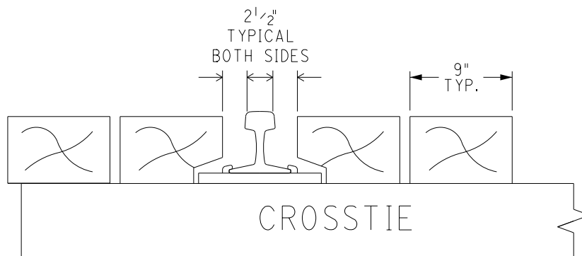
NON-SHIMMED DETAIL
