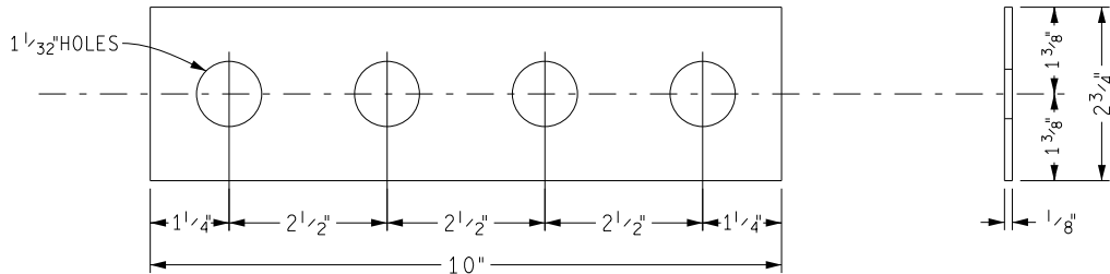
10552 SPLICE PLATE, FIBRE
