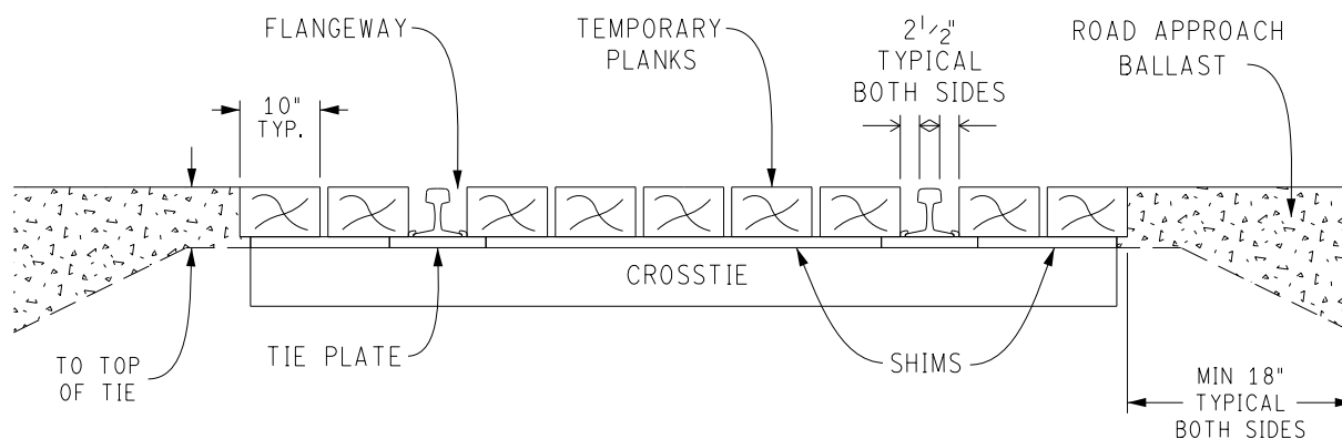
SHIMMED DETAIL
