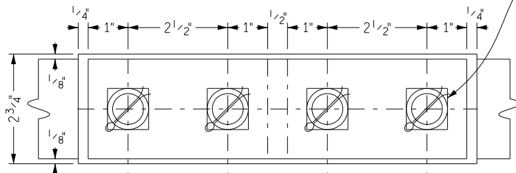
TYPE 2 SWITCH ROD INSTALLATION
