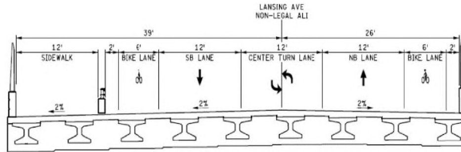
PROPOSED BRIDGE SECTION SECTION A-A
