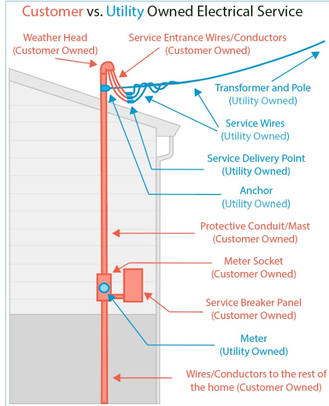
Figure 1. Illustrative Diagram of Electric Service Components 2
