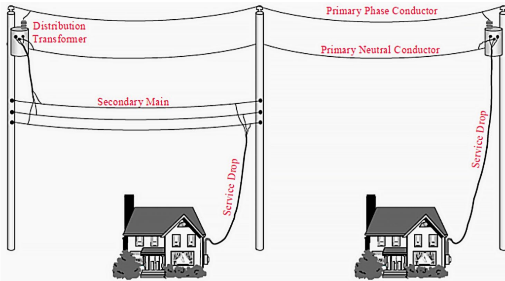
Figure 2. Transformer, Secondary, and Service Conductor Illustration 4
