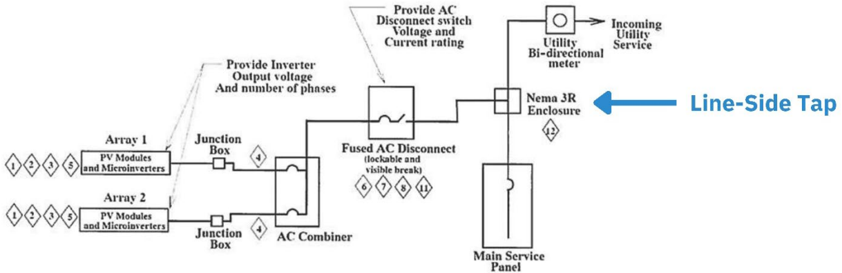
Figure 3. Line-Side Tap PV Connection Between Utility Meter and Main Service Panel
