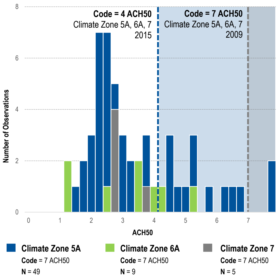
Figure 1.10: ACH50 Values Climate Zone 5A, 6A, 7
