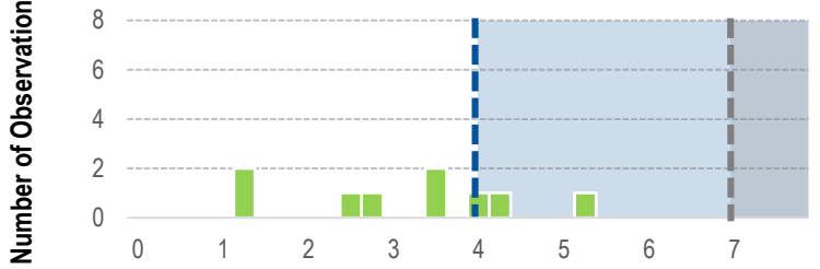
Figure 1.13: ACH50 Values Climate Zone 7
