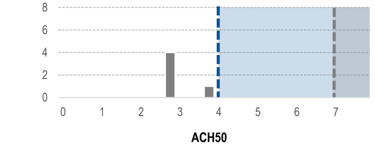
Figure 1.13: ACH50 Values Climate Zone 7
