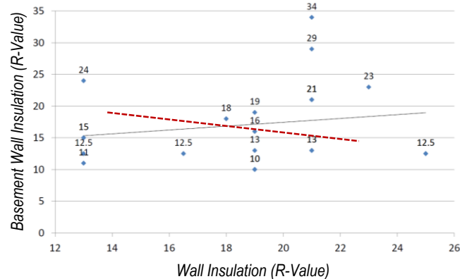
Figure 1.18: Wall R vs. Basement R 1
