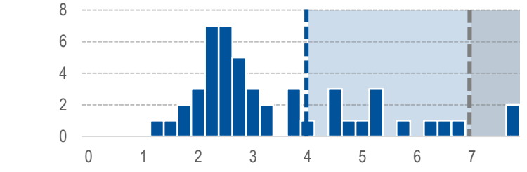
Figure 1.12: ACH50 Values Climate Zone 6A
