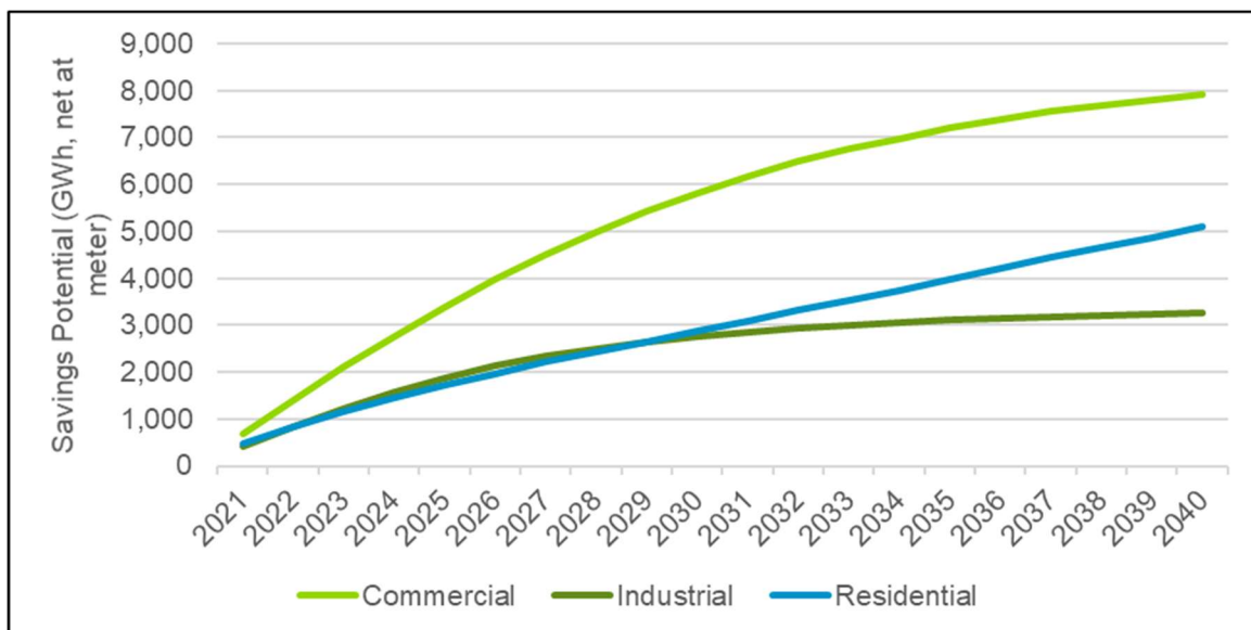
Figure 9-1. Lower Peninsula EWR Cumulative Achievable Potential, Incremental Annual Electricity Savings by Sector, Reference Scenario (GWh, Net at Meter)
