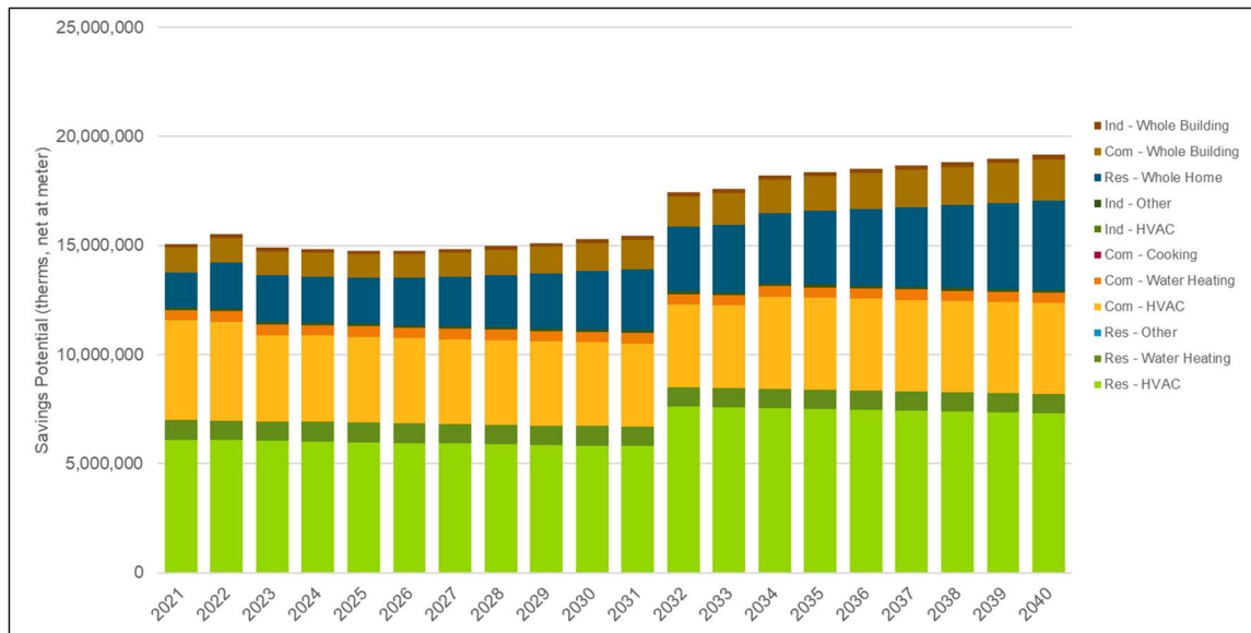
Figure 6-12. Upper Peninsula EWR Economic Potential, Natural Gas by End Use Reference Scenario (therms, Net at Meter)
