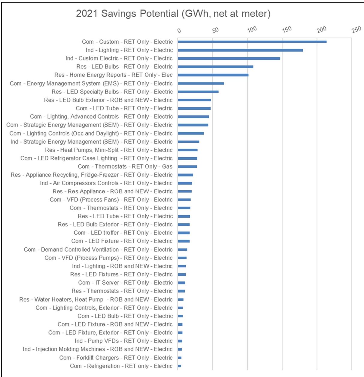
Figure 9-19. Lower Peninsula EWR Achievable Potential, 2021 Top Measures for Electricity Savings, Reference Scenario (GWh, Net at Meter)
