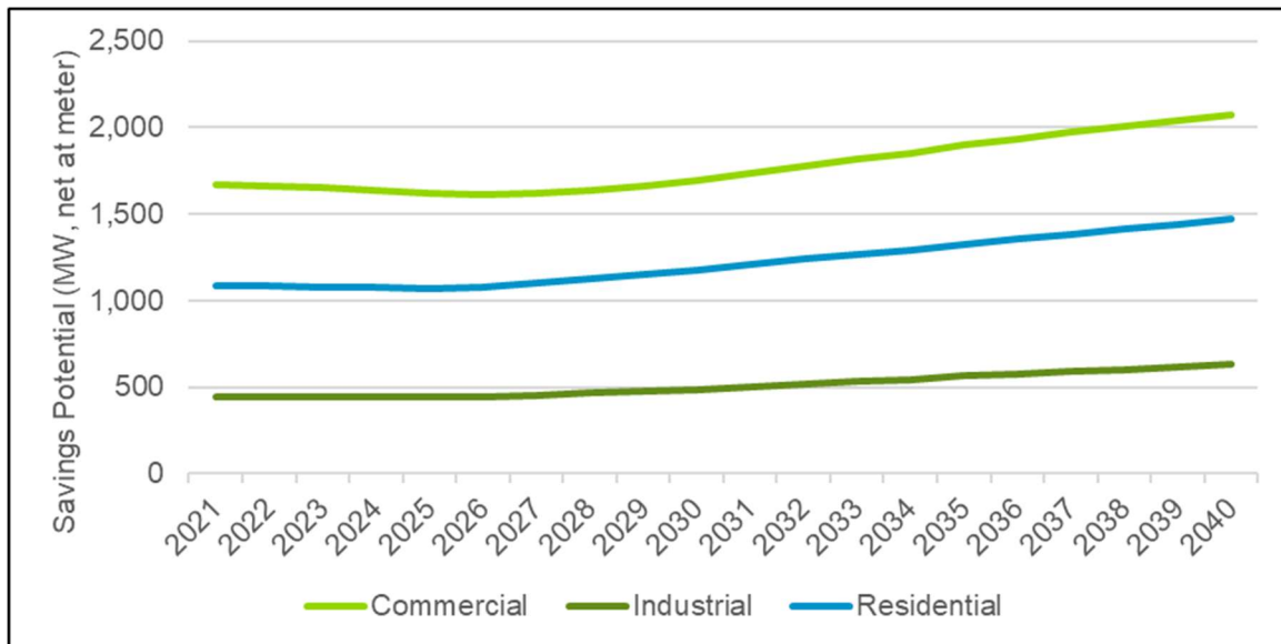
Figure 5-3. Lower Peninsula EWR Technical Potential, Summer Peak Demand Savings by Sector, Reference Scenario (MW, Net at Meter)
