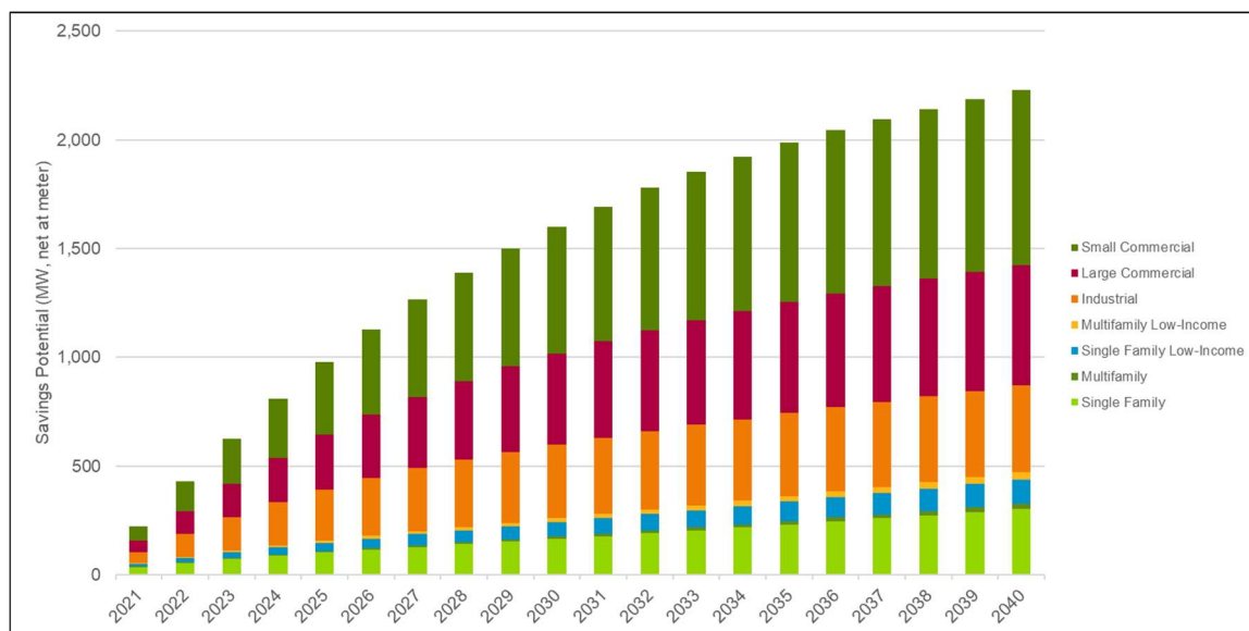
Figure 9-15. Lower Peninsula EWR Cumulative Achievable Potential, Incremental Annual Summer Peak Demand Savings by Customer Segment, Reference Scenario (MW, Net at Meter)
