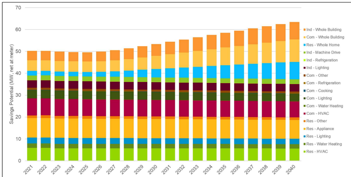
Figure 6-8. Upper Peninsula EWR Economic Potential, Electricity Savings by End Use, Reference Scenario (GWh, Net at Meter)
