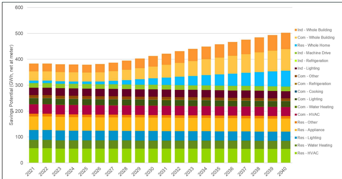
Figure 5-8. Upper Peninsula EWR Technical Potential, Electricity Savings by End Use. Reference Scenario (GWh, Net at Meter)
