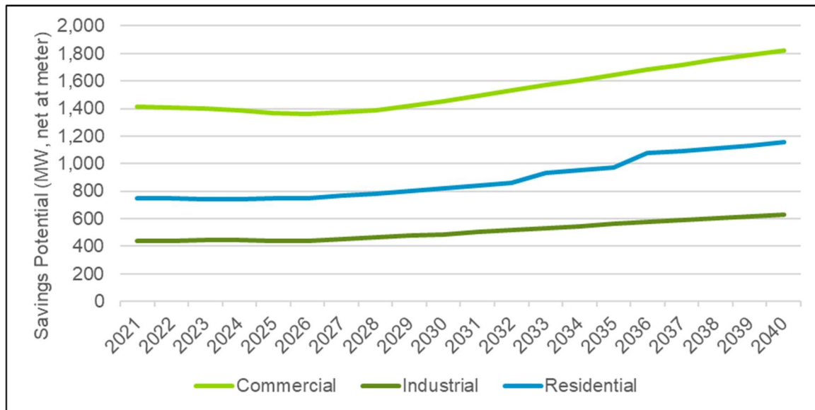
Figure 6-3. Lower Peninsula EWR Economic Potential, Summer Peak Demand Savings by Sector, Reference Scenario (MW, Net at Meter)
