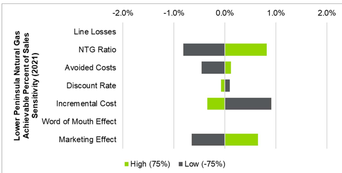
Figure 9-27. Lower Peninsula Natural Gas Achievable Percent of Sales Sensitivity 1 Reference Scenario (2021)
