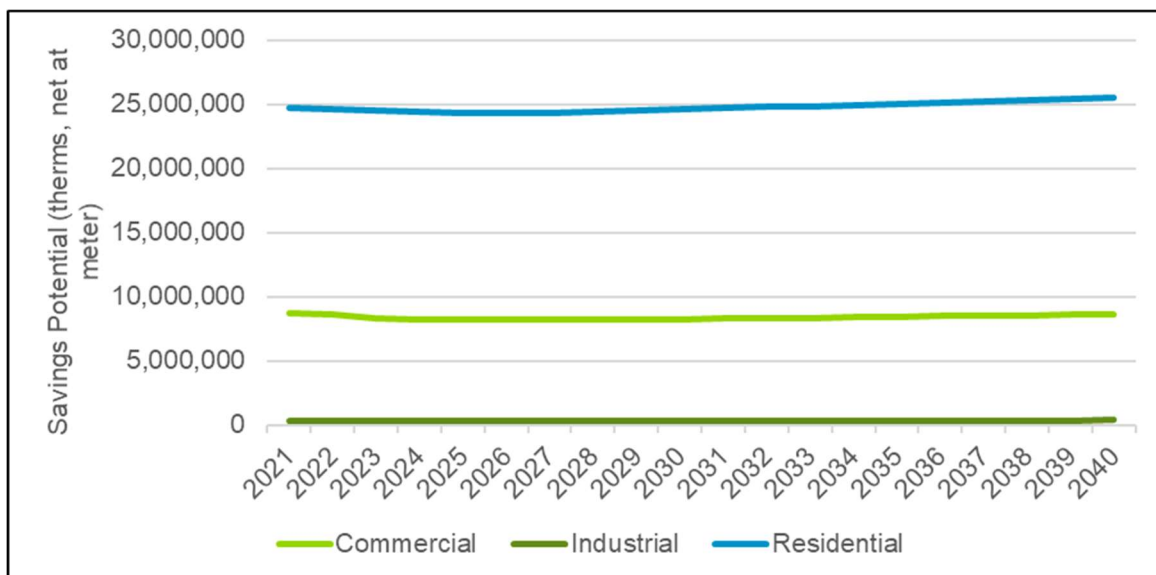
Figure 5-6. Upper Peninsula EWR Technical Potential, Natural Gas Savings by Sector, Reference Scenario (therms, Net at Meter)
