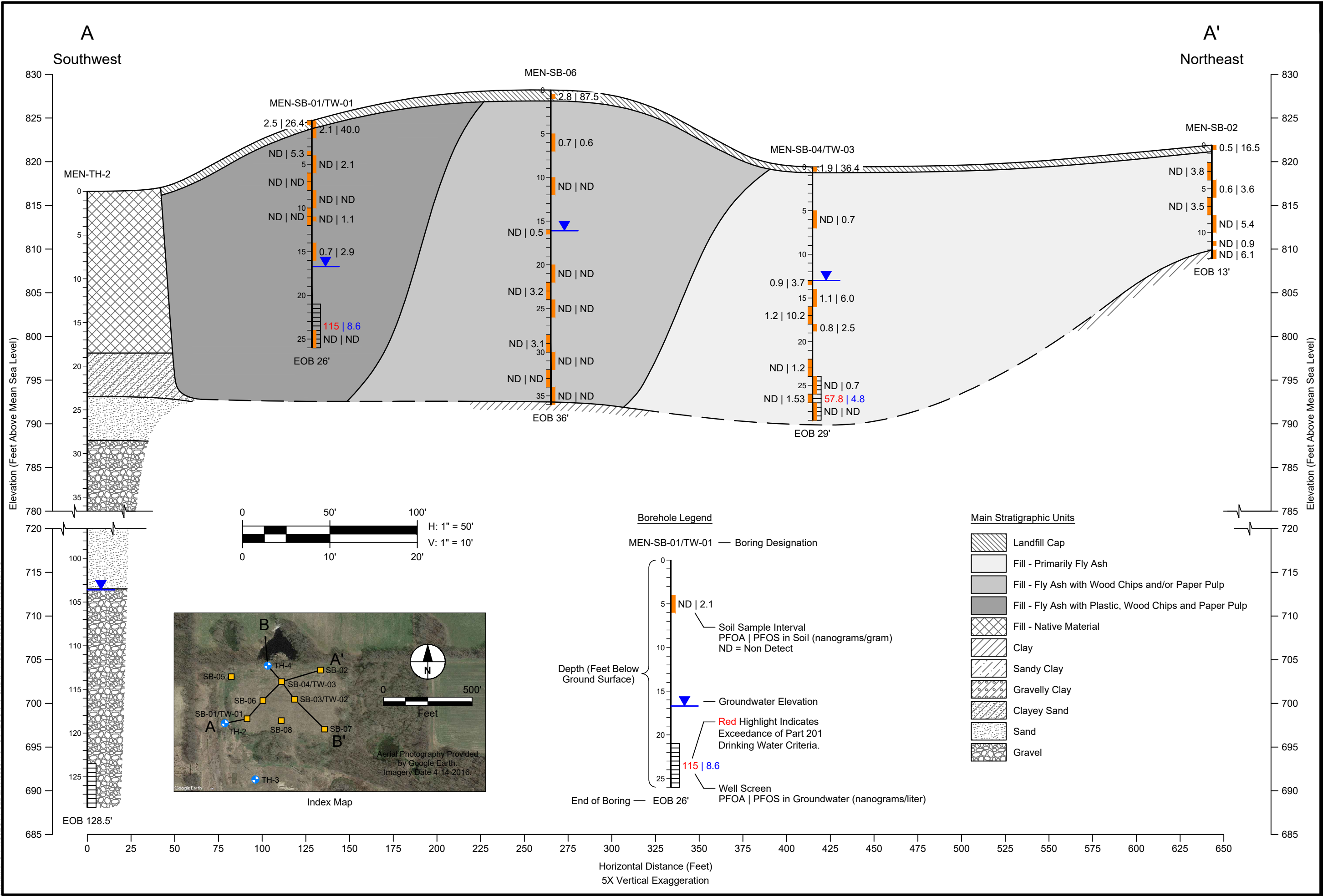
GEOLOGIC CROSS SECTION A - A'
