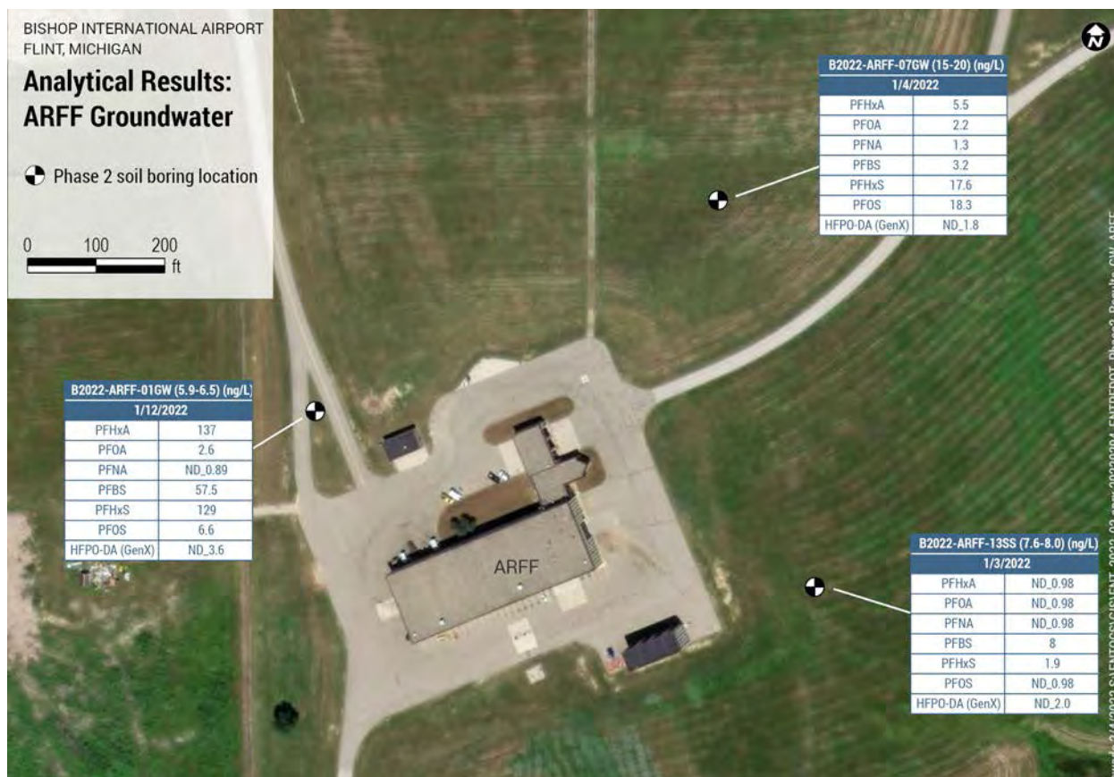
Figure 3-6. Phase 2 Groundwater Sampling Results at the ARFF Station Area (ND = not detected).
