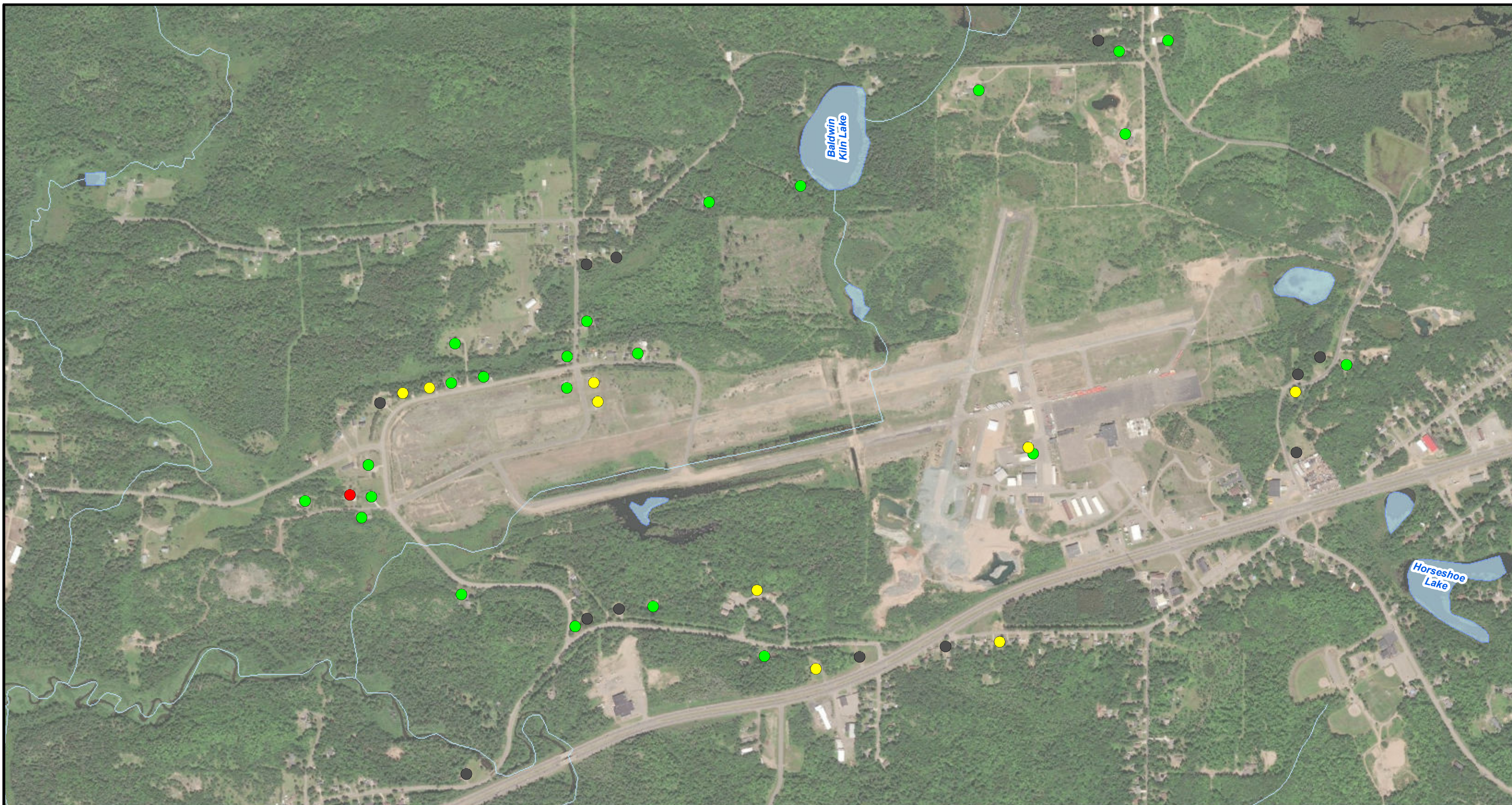
FIGURE 1 RESIDENTIAL WELL SAMPLING RESULTS PFAS HEAT MAP
