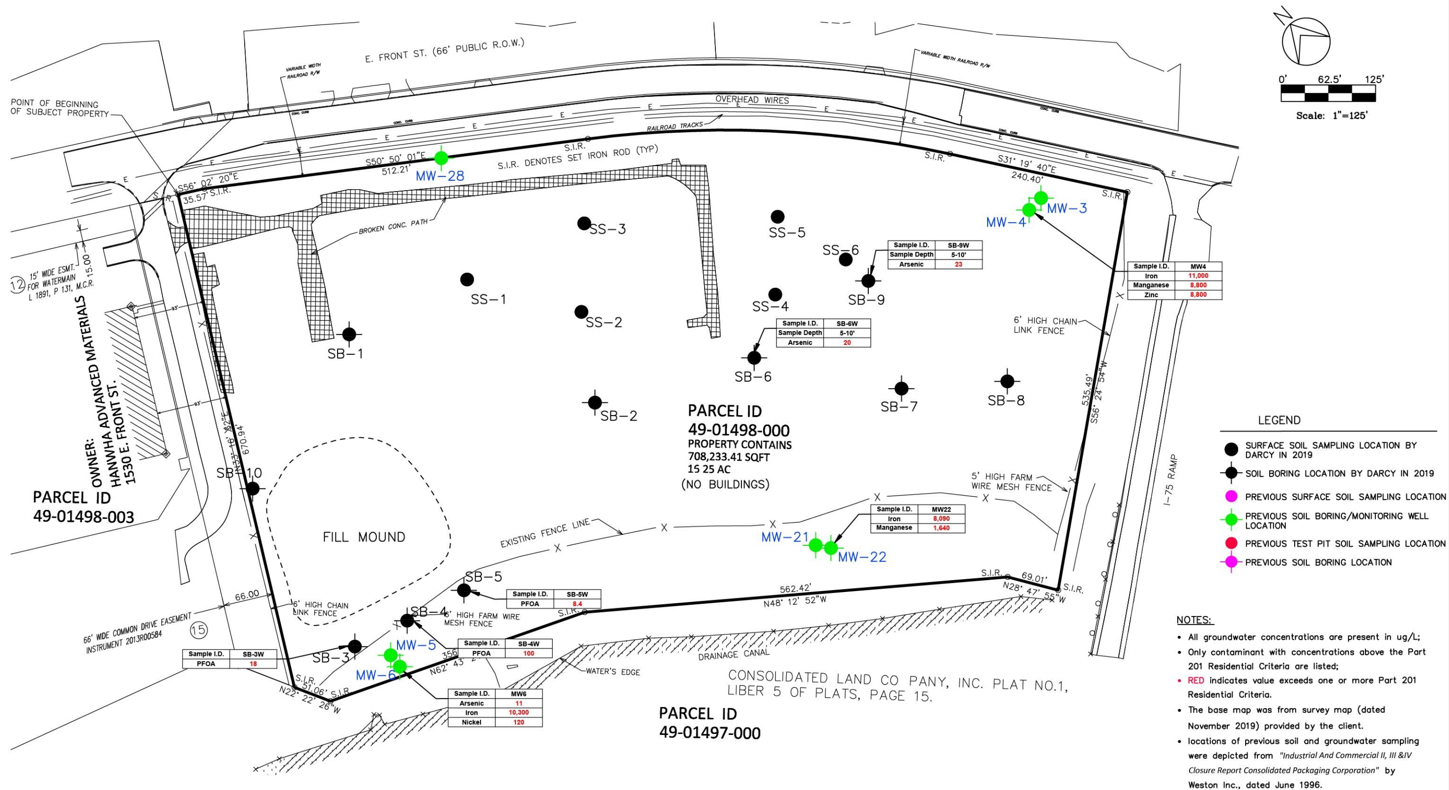
FIGURE 5: CONTAMINANTS CONCENTRATIONS IN GROUNDWATER SAMPLE 1700 EAST FRONT STREET MONROE, MICHIGAN
