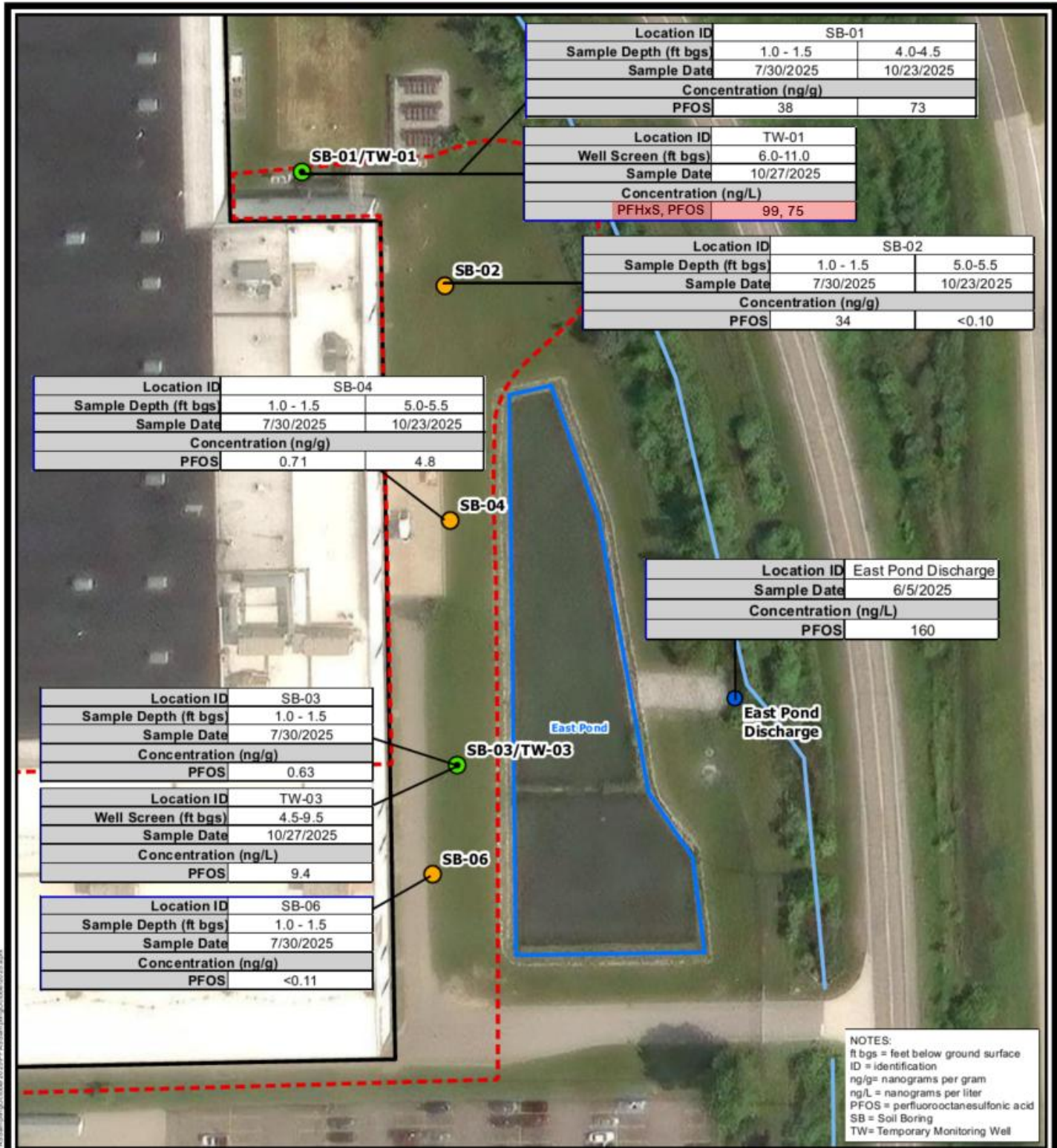
FIGURE 1 SOIL, GROUNDWATER, AND EAST POND DISCHARGE SAMPLING RESULTS MAP
