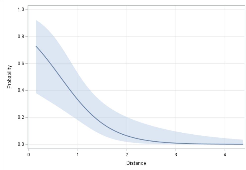
Figure 12. Muscle Logistic Regression Model for Oscoda area deer (sampled in 2018 and 2020) (Group 1= PFOS detected in liver sample)
