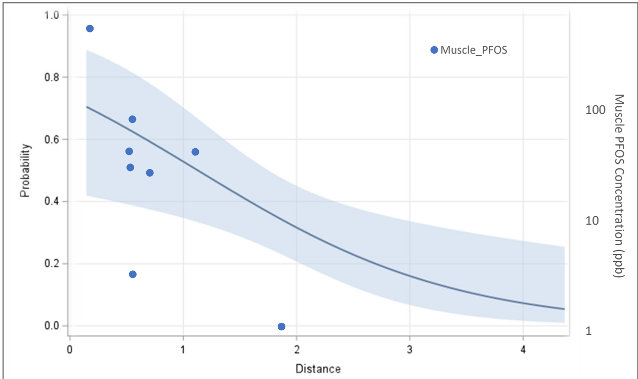
Figure 14. Liver PFOS Logistic Regression Model with Muscle PFOS Concentrations (ppb – logarithmic scale) for Oscoda area deer sampled in 2018 and 2020
