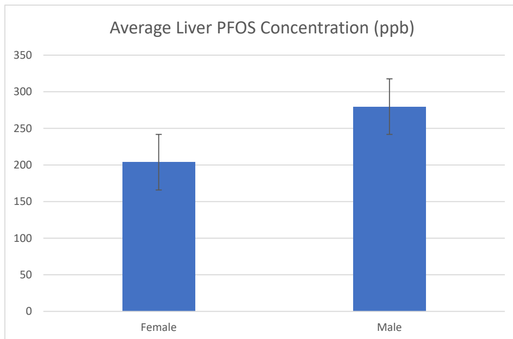
Figure 19. Average Liver PFOS Concentration (parts per billion [ppb] or nanograms per gram [ng/g]) of Oscoda Area Deer in 2018 and 2020
