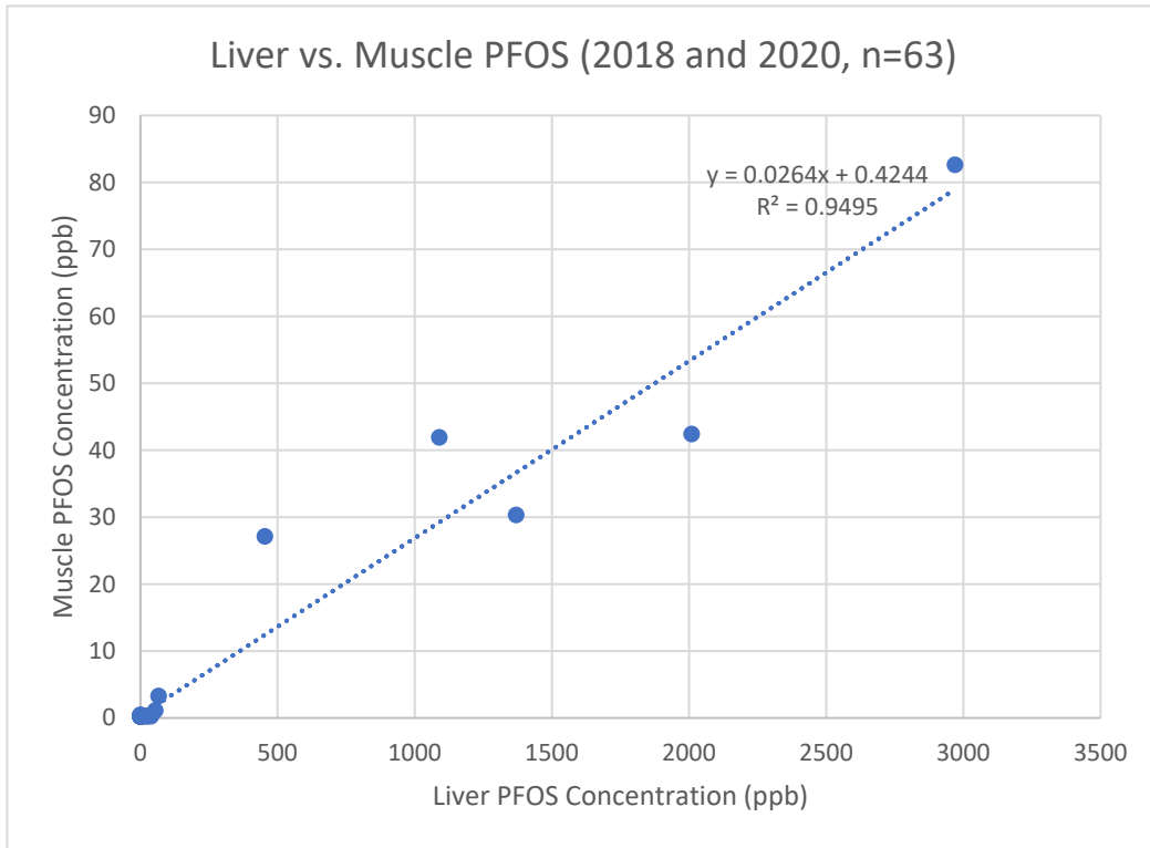
Figure 8. Comparison of liver and muscle PFOS excluding non-detects (in parts per billion [ppb] or nanograms per gram [ng/g]) from deer samples collected in 2018 and 2020 from Iosco County
