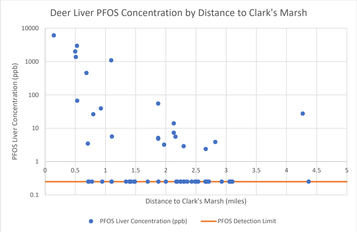
Figure 2: Individual deer liver PFOS levels (in parts per billion [ppb] or nanograms per gram [ng/g]) by distance of the deer collection locations from Clark's Marsh. This includes deer that were collected in 2018 and 2020. The orange line is set at 0.25 ppb, which is the detection limit. Points on the line are liver samples that did not have a detection of PFOS.
