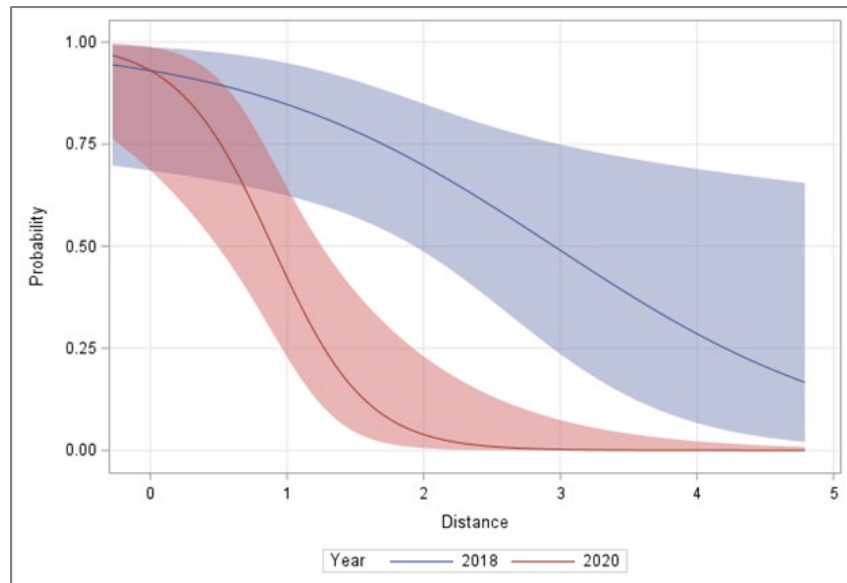
Figure 16. Logistic Regression for Liver PFOS Detection by Miles from Clark's Marsh, by year – 2018 and 2020
