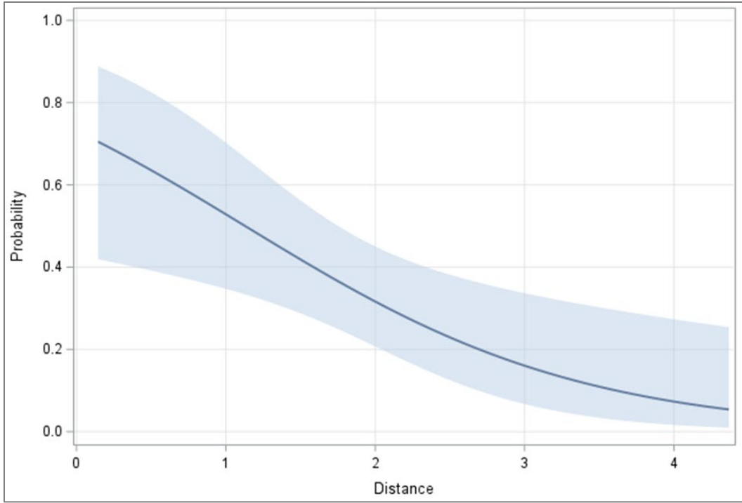
Figure 3: Modeled probability (shaded area is the 95% upper and lower confidence limits) for a detection of PFOS in liver and distance in miles from Clark’s Marsh.
