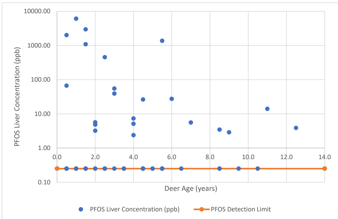
Figure 17. Oscoda area deer liver PFOS concentration (ppb) by deer age, 2018 and 2020
