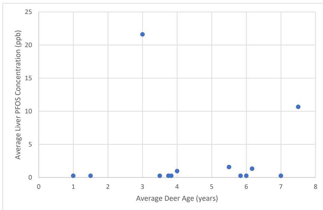
Figure 18. Family group average liver PFOS concentrations (in parts per billion [ppb] or nanograms per gram [ng/g]) by average age from samples collected in 2018 and 2020
