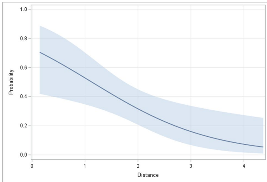
Figure 11. Liver PFOS Logistic Regression Model (Predicted Probabilities) for Oscoda area deer sampled in 2018 and 2020 (Detect Status 1 = PFOS detected in liver sample)
