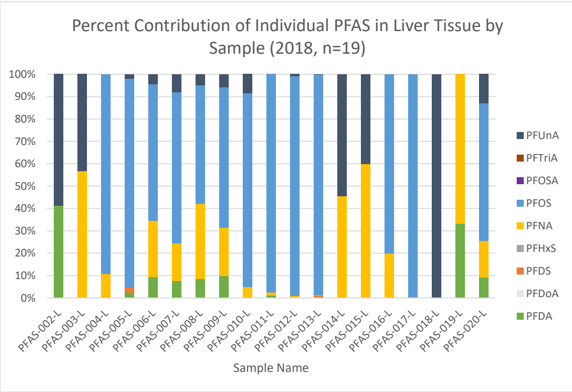
Figure 4: Contribution of individual PFAS in deer with liver detections for \geq 1 PFAS from deer samples collected in 2018 from losco County
