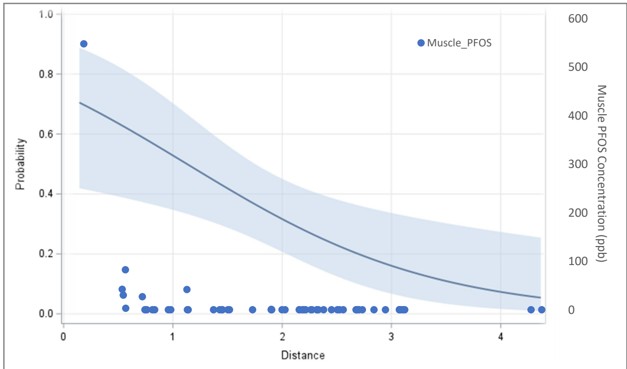
Figure 13. Liver PFOS Logistic Regression Model with Muscle PFOS Concentrations (ppb) for Oscoda area deer sampled in 2018 and 2020
