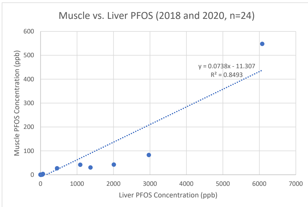
Figure 8. Comparison of liver and muscle PFOS excluding non-detects (in parts per billion [ppb] or nanograms per gram [ng/g]) from deer samples collected in 2018 and 2020 from Iosco County
