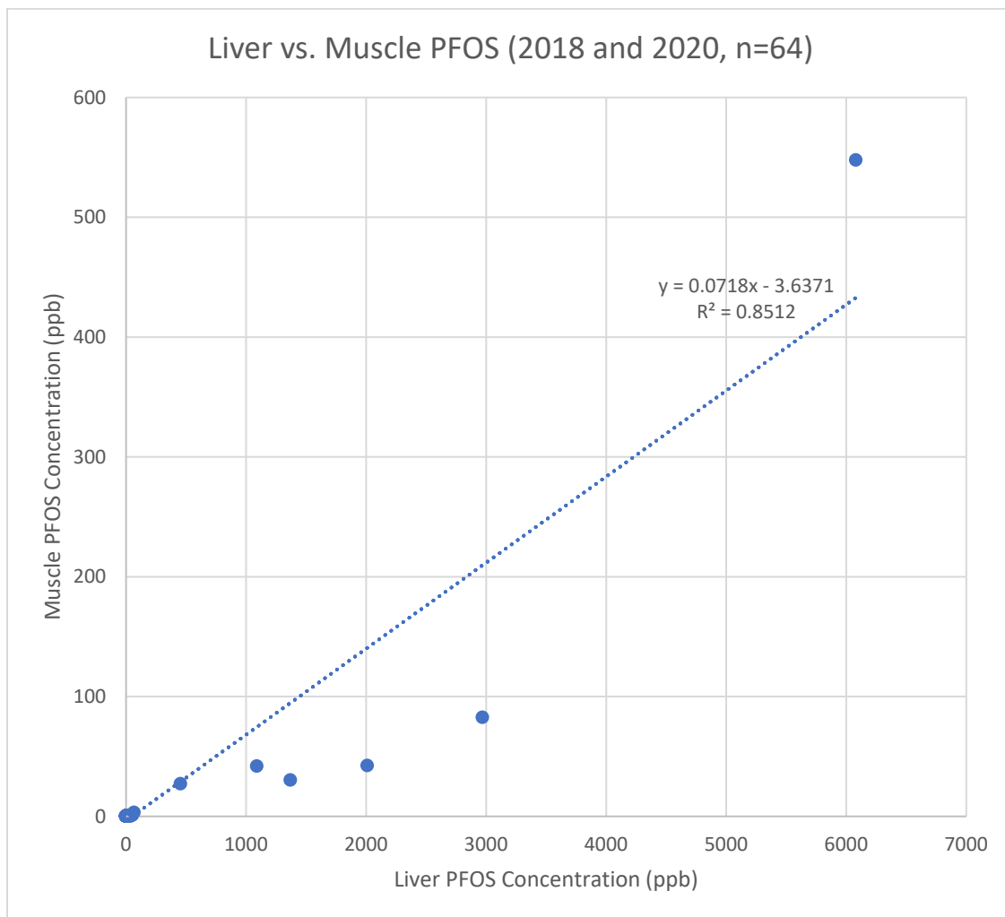
Figure 6. Comparison of liver and muscle PFOS (in parts per billion [ppb] or nanograms per gram [ng/g]) from deer samples collected in 2018 and 2020 from Iosco County
