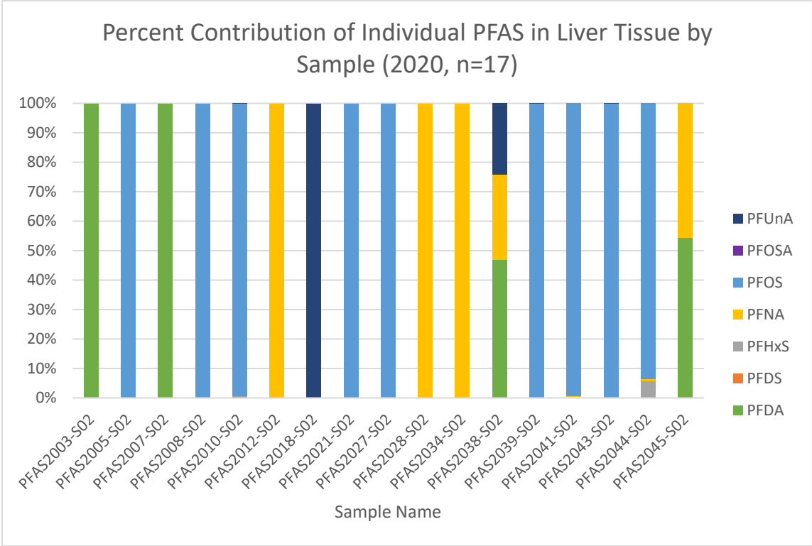
Figure 5: Contribution of individual PFAS in deer with liver detections for \geq 1 PFAS from deer samples collected in 2020 from Iosco County
