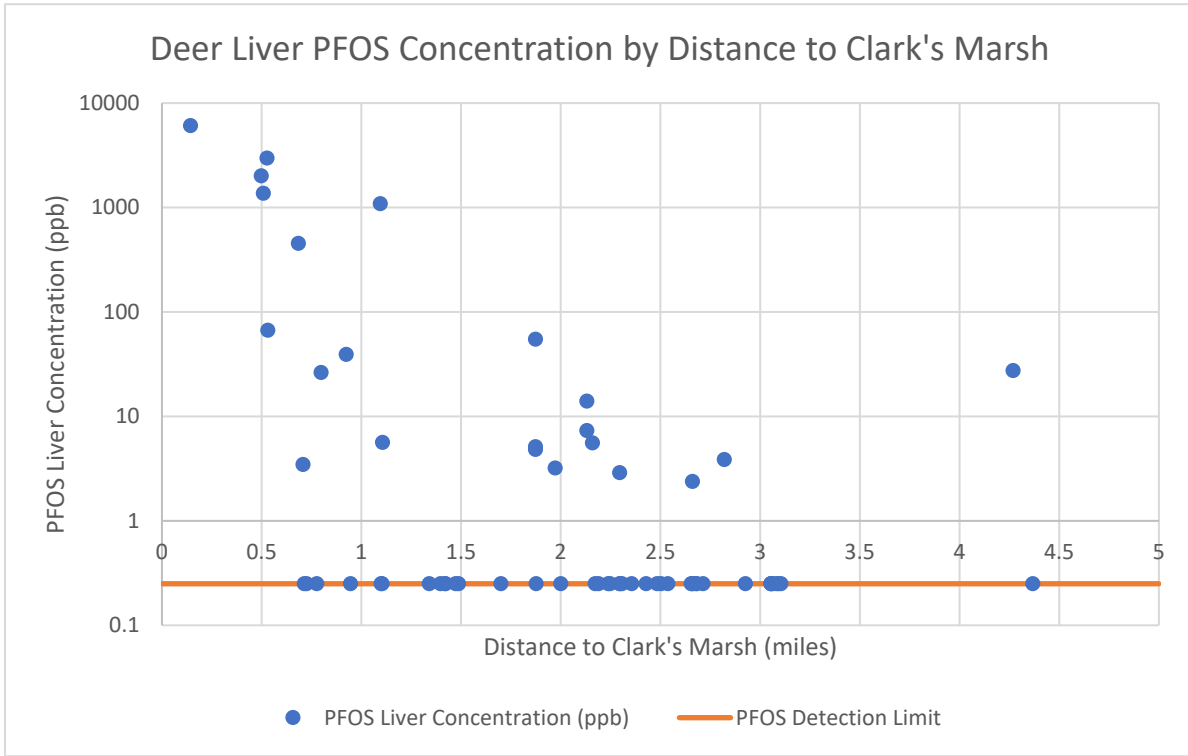
Figure 10. Log scale of deer liver PFOS concentration (in parts per billion [ppb] or nanograms per gram [ng/g]) by distance from Clark's Marsh (in miles) from deer samples collected in 2018 and 2020 from the Oscoda area
