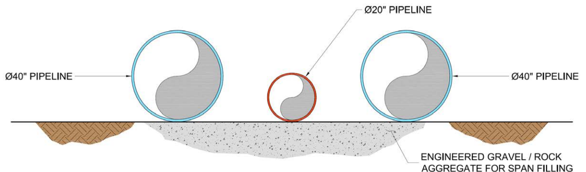
Figure 21: HDPE pipelines.
