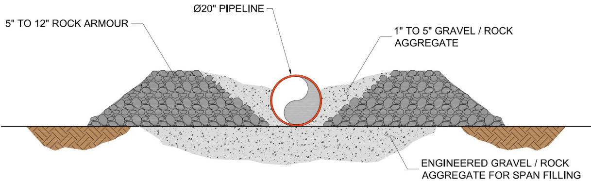
Figure 18: Gravel/rock berm.
