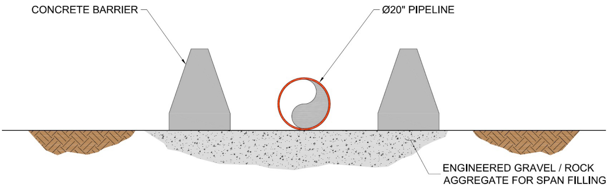
Figure 19: Concrete barrier.
