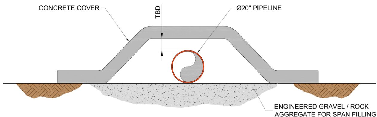
Figure 24: Concrete cover.
